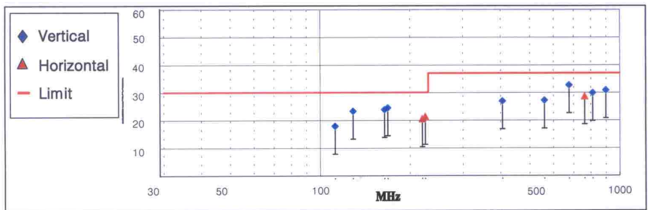
< Fig 6. Radiated emission result >
