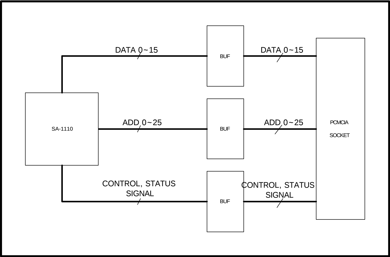
PCMCIA PATH BLOCK DIAGRAM
