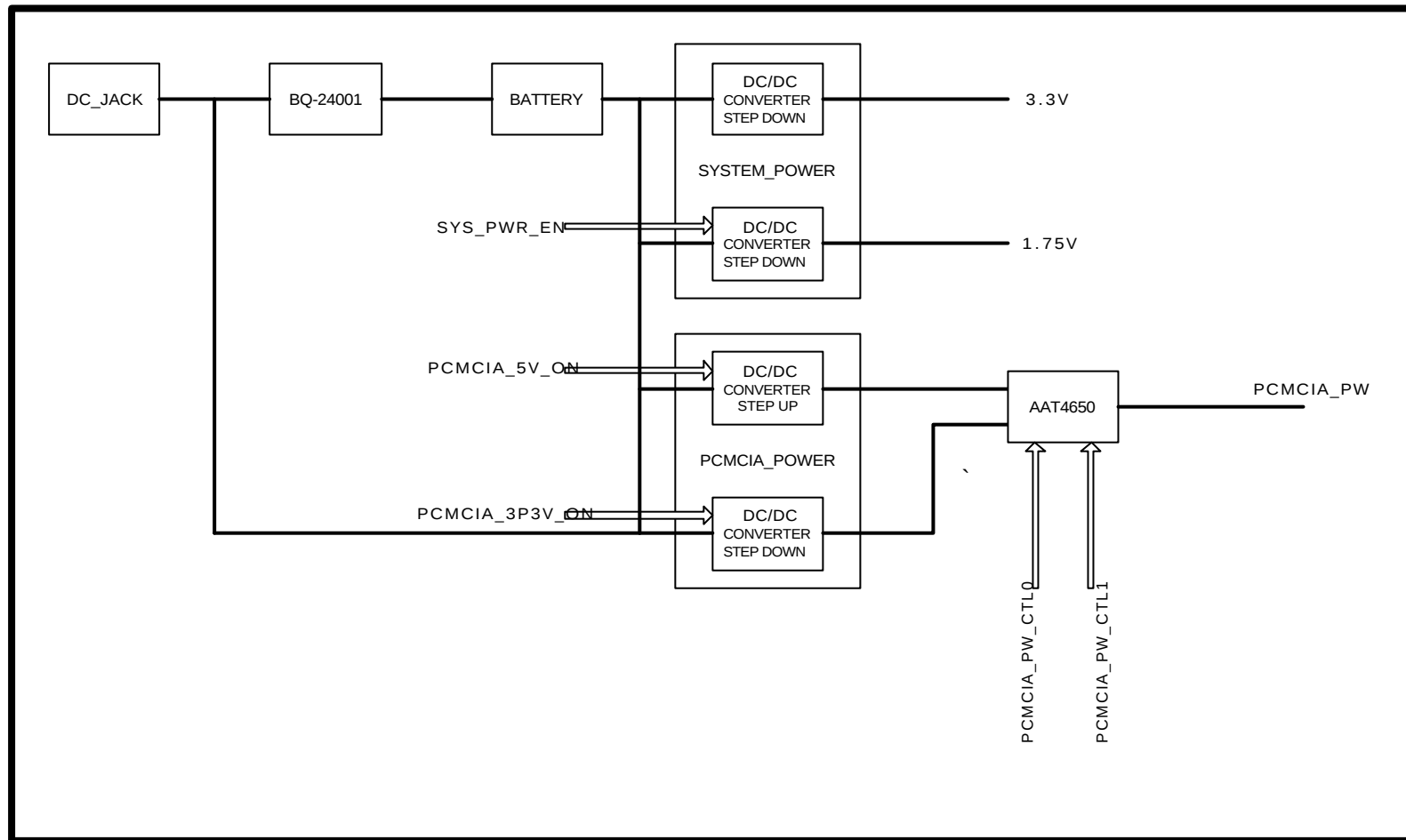
MAIN POWER BLOCK DIAGRAM
