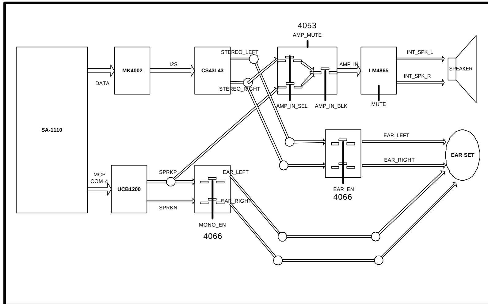
AUDIO PATH BLOCK DIAGRAM
