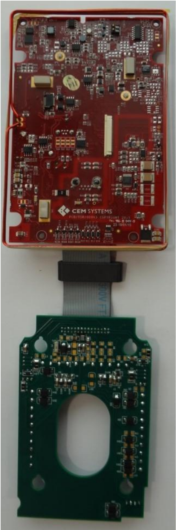
All 3 boards assembled without case, Front View
