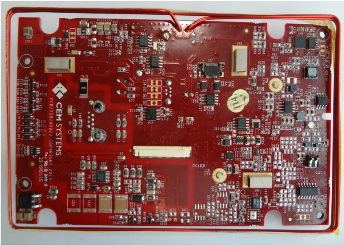
Main Board Rear View
