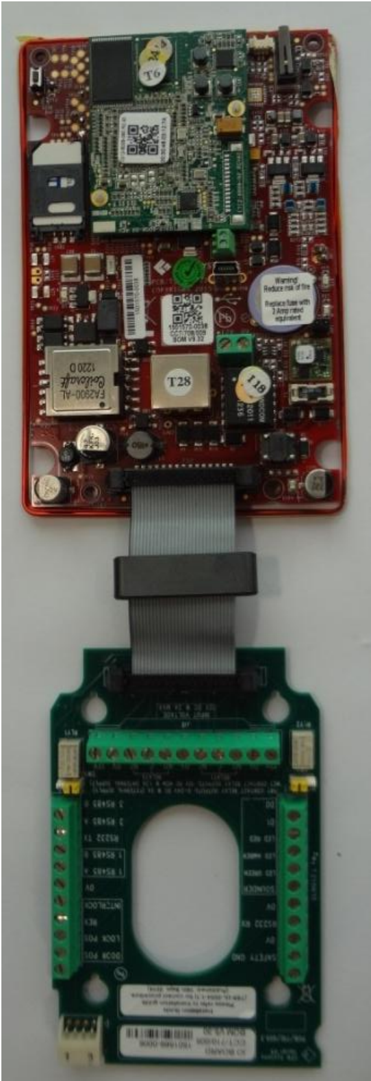
All 3 boards assembled without case, Front View
