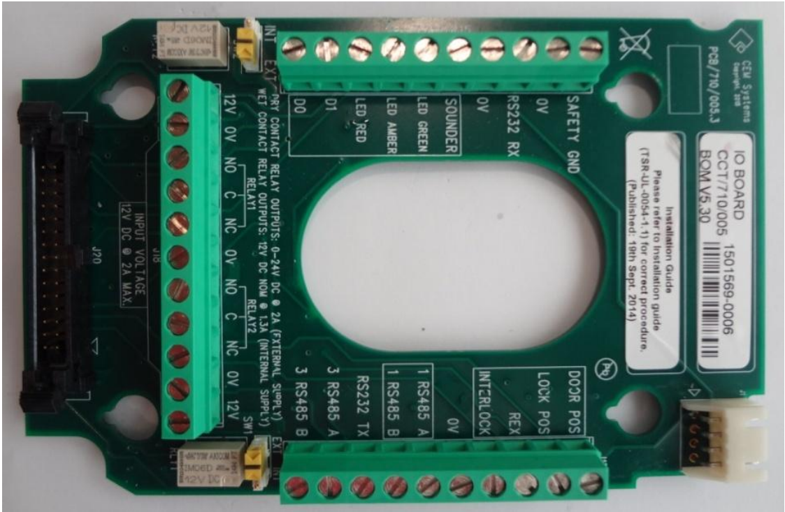
I/O Board Front View
