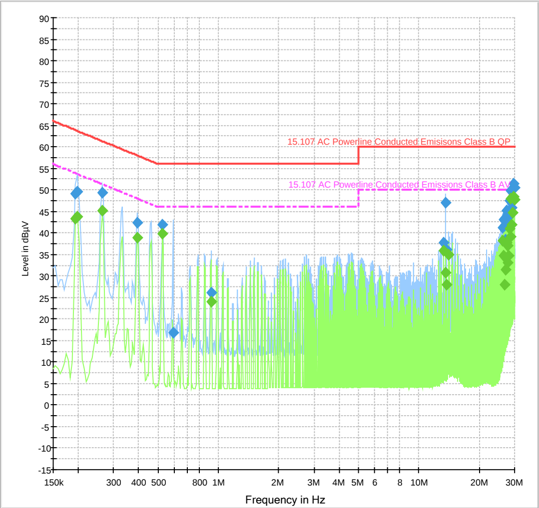
FCC Class B Conducted emissions on Mains 150kHz-30MHz ESHS10 + UH396 Rx prescans
