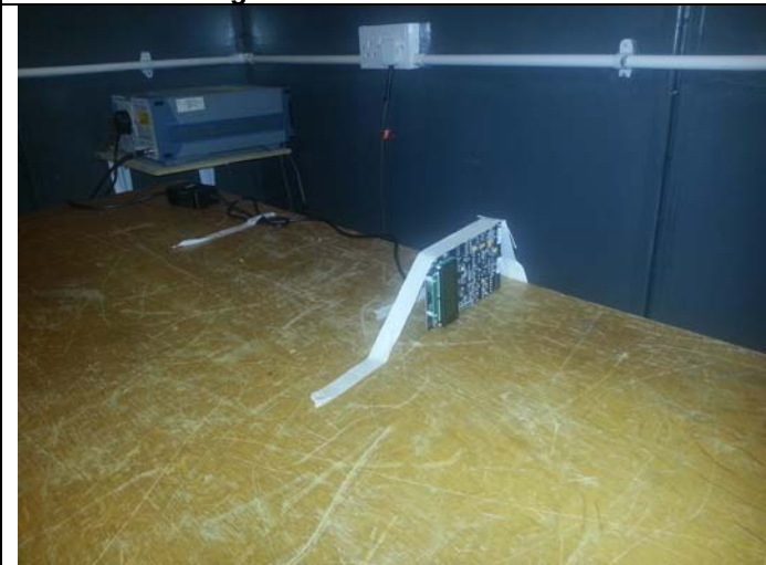
Fig 3 Radiated Emissions -
