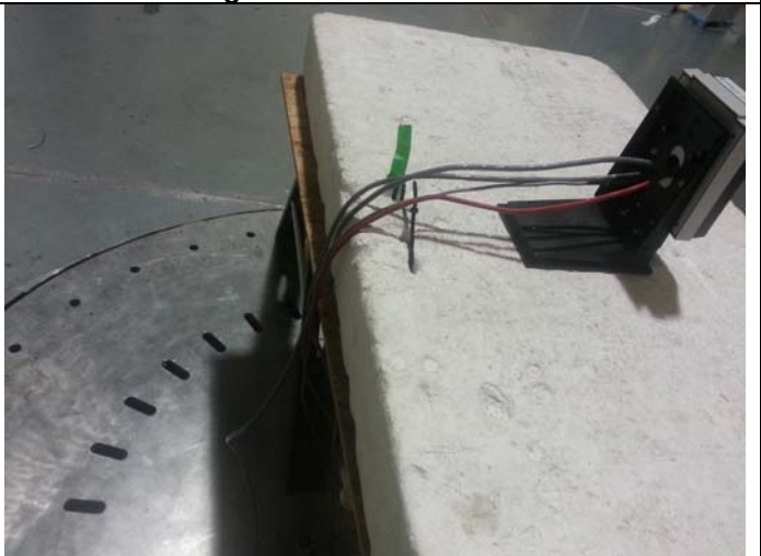
Fig 2 Radiated Emissions
