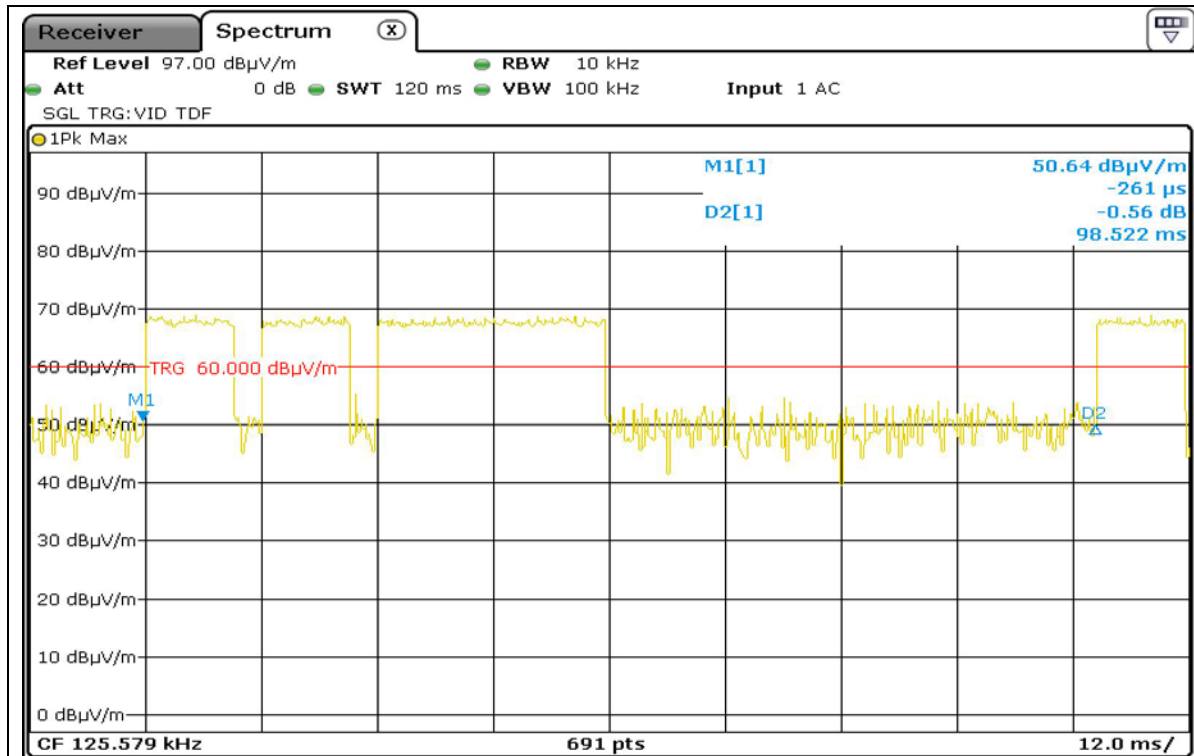
Fig 3 Duty Cycle 125KHz
