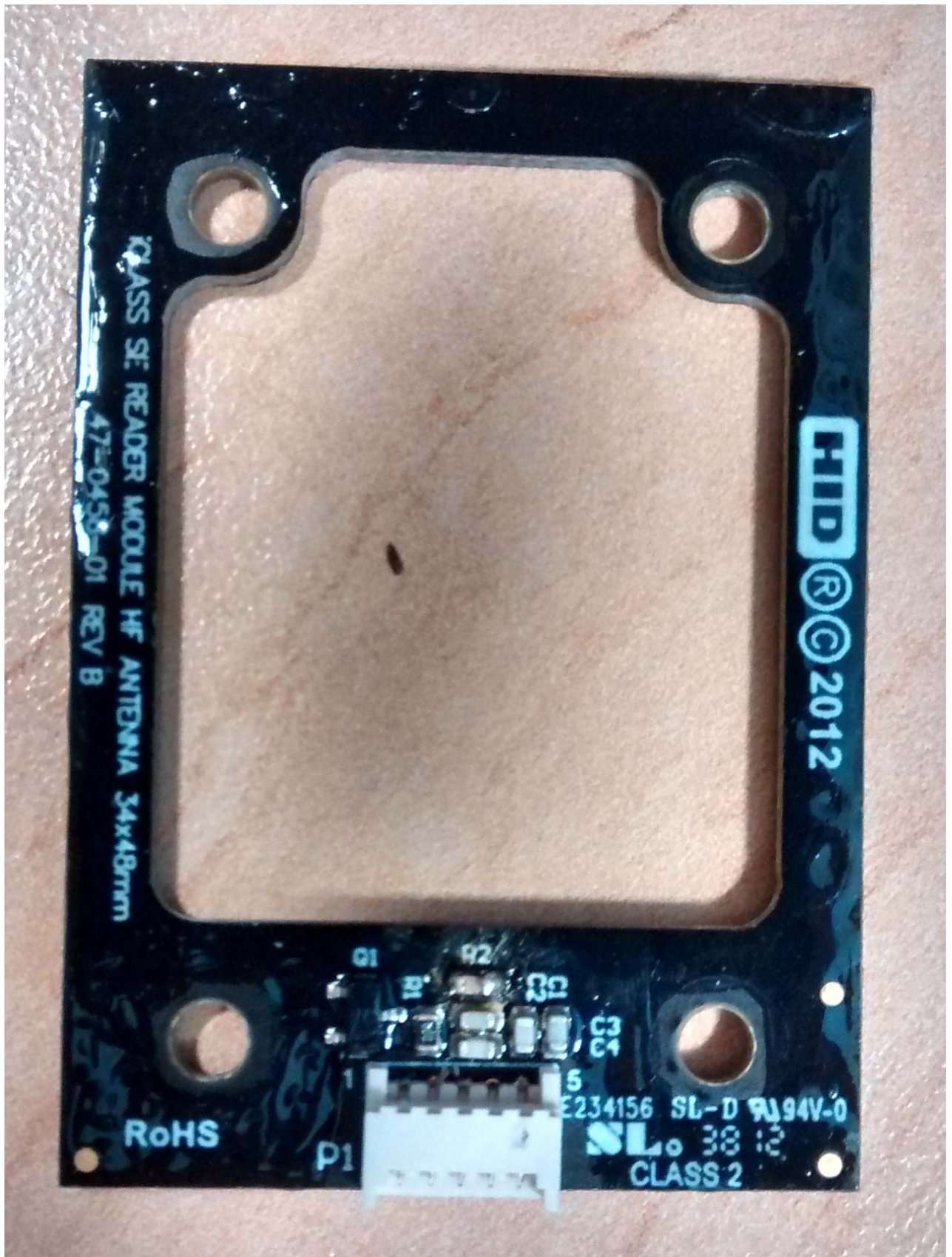
Individual pcbs; HF antenna back view
