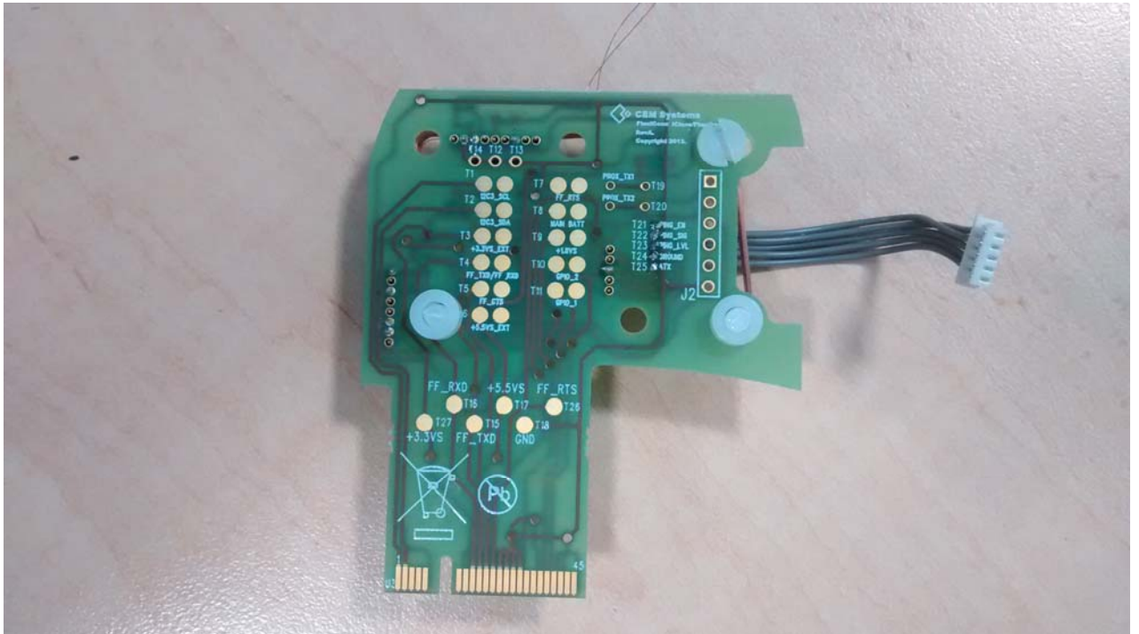
Individual pcbs; main pcb Side A
