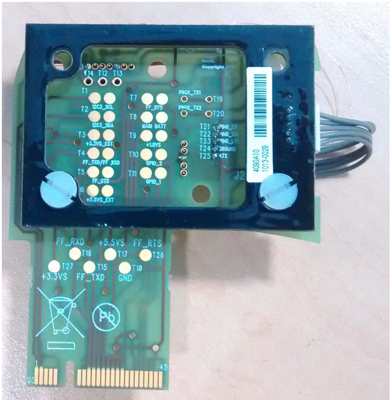
Assembled pcbs; top view
