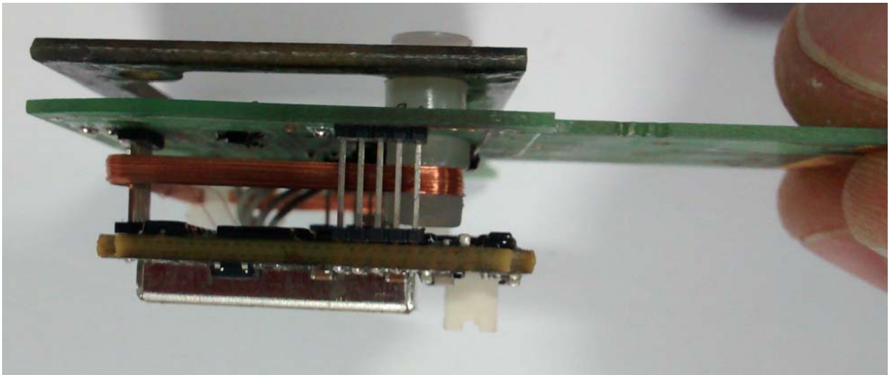
Assembled pcbs; side view
