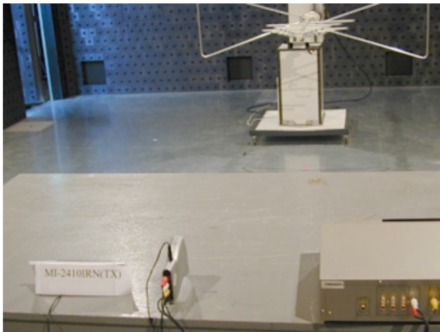
Photo 2: Spurious Set-up
