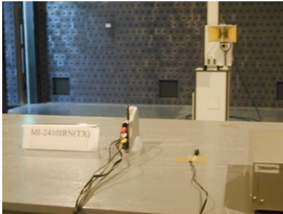
Photo 3: Spurious Set-up
