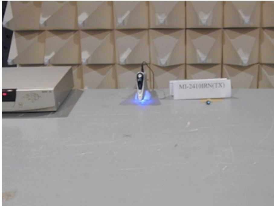
Photo 1: Spurious Set-up
