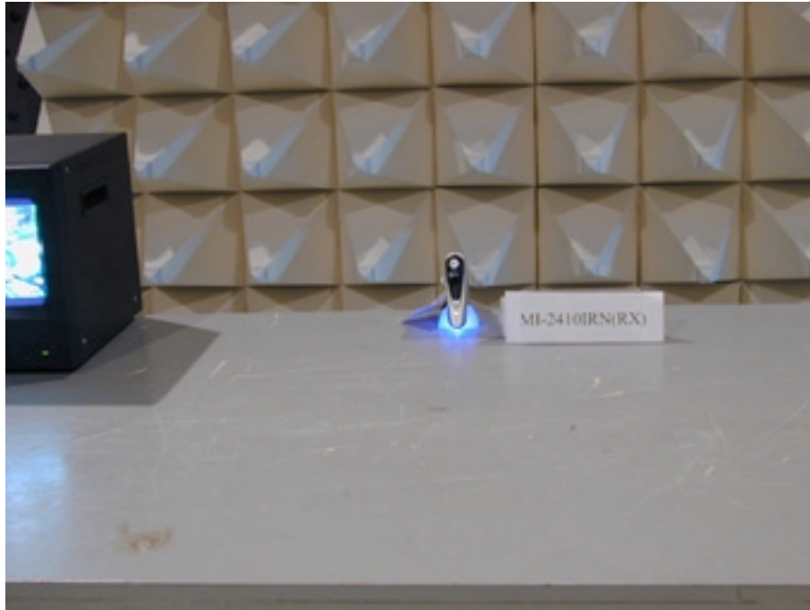
Photo 1: Spurious Set-up
