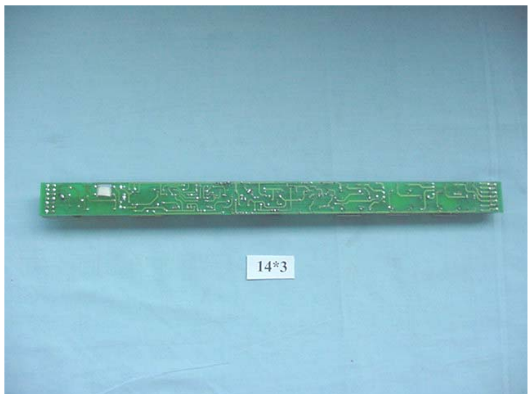
FIGURE 3 BALLAST (M/N: FBT T5 14x3) MAIN BOARD (SOLDERED SIDE)
