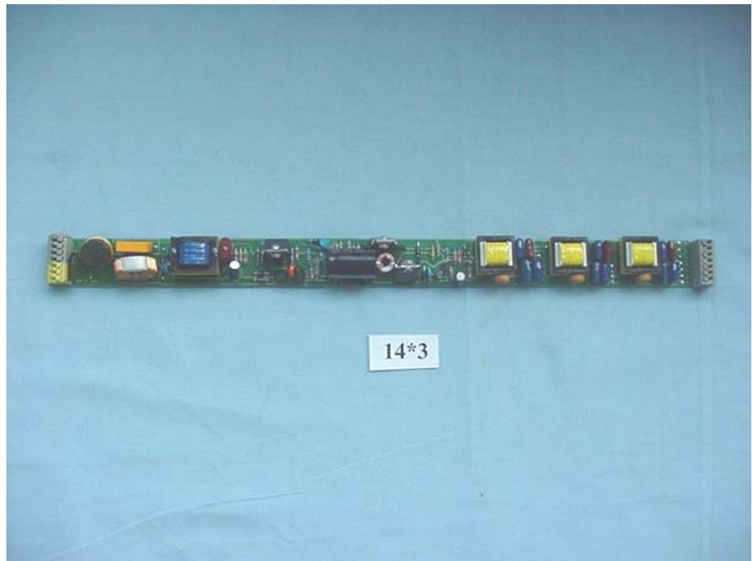
FIGURE 2 BALLAST (M/N: FBT T5 14x3) MAIN BOARD (COMPONENT SIDE)
