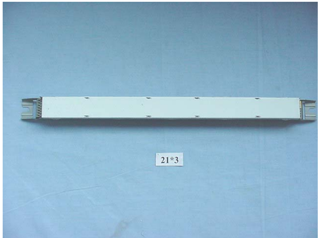
Figure 3 BALLAST (M/N: FBT T5 21x3) GENERAL APPEARANCE (FRONT VIEW)
