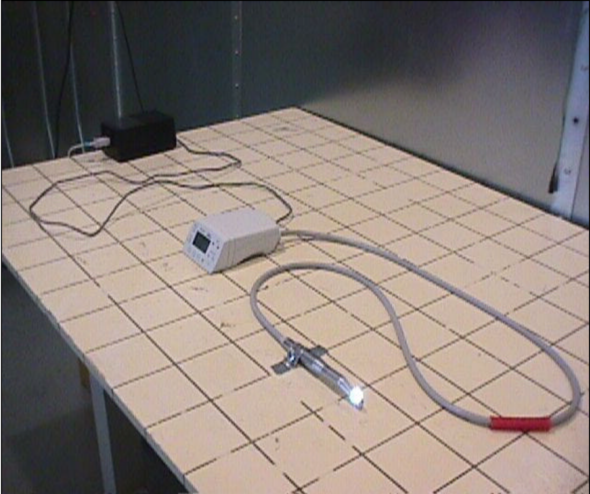
Photo of the Conducted Emissions Test
