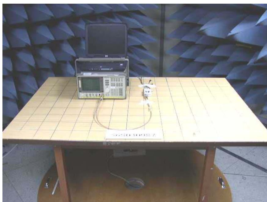
Number of Hopping Frequencies Measurement Test Setup
