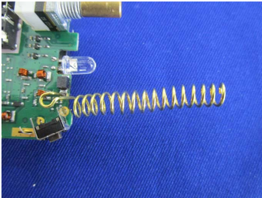
EUT – Two-way Radio Antenna View
