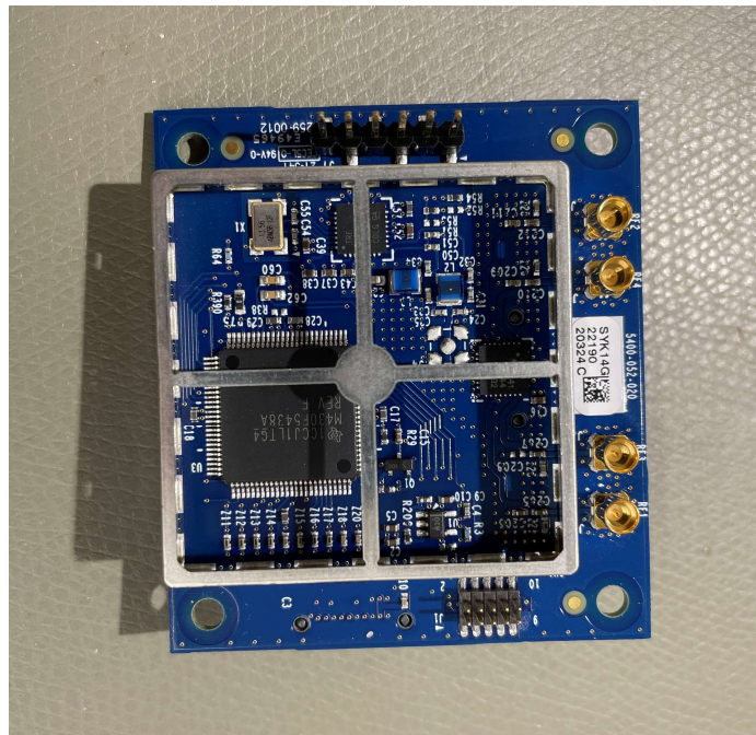
Figure 5. RF Module PCBA Top View without cover
