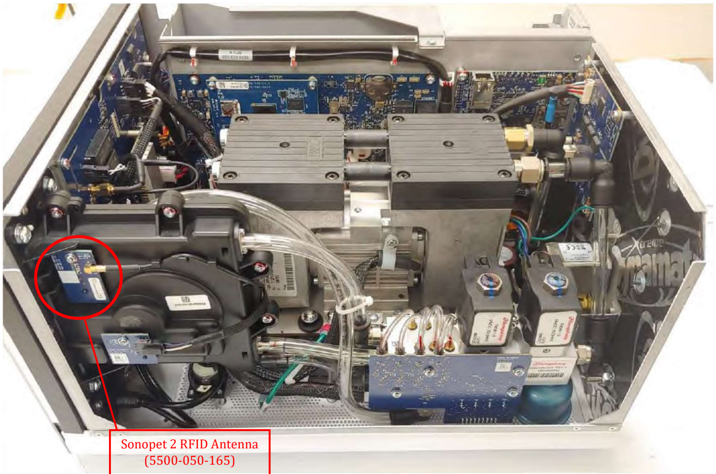
Figure 2. Internal Right View
