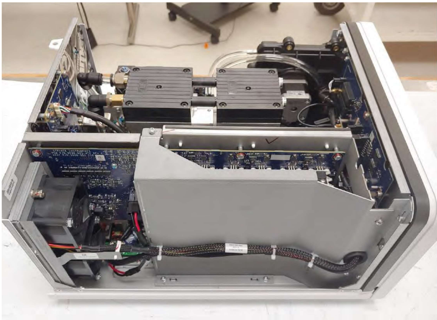
Figure 3. Internal Left View
