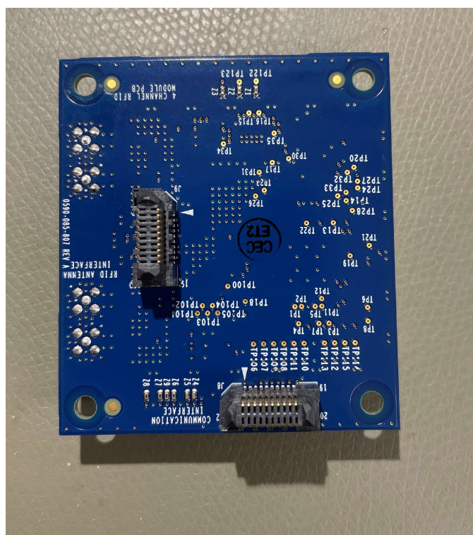
Figure 6. RF Module PCBA Bottom View
