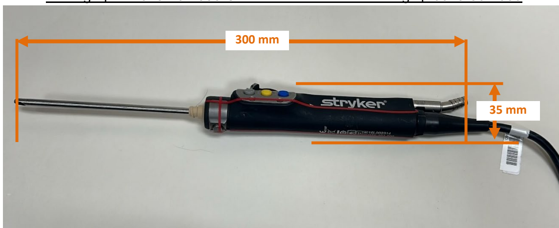
Photograph 2: 375-704-500 Overall Dimensions including tip 0375-562-000
