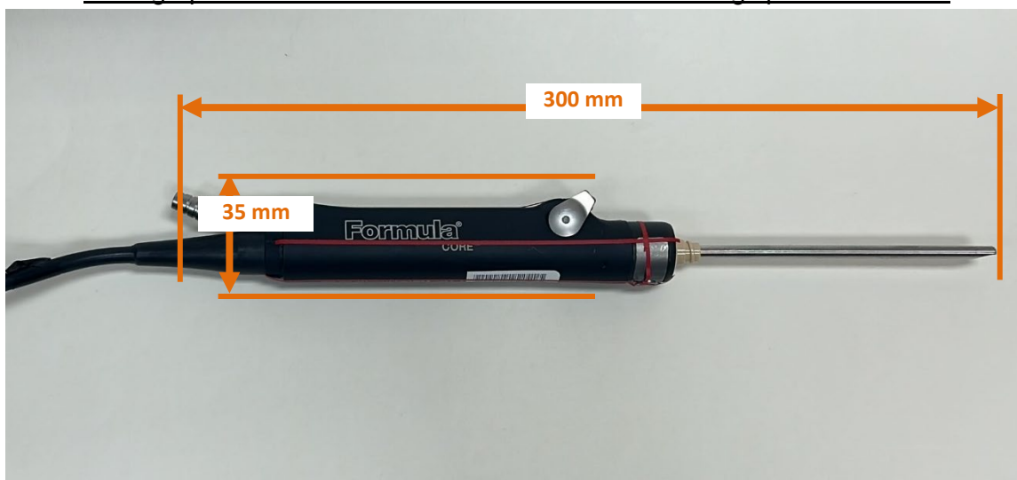
Photograph 1: 375-701-500 Overall Dimensions including tip 0375-562-000
