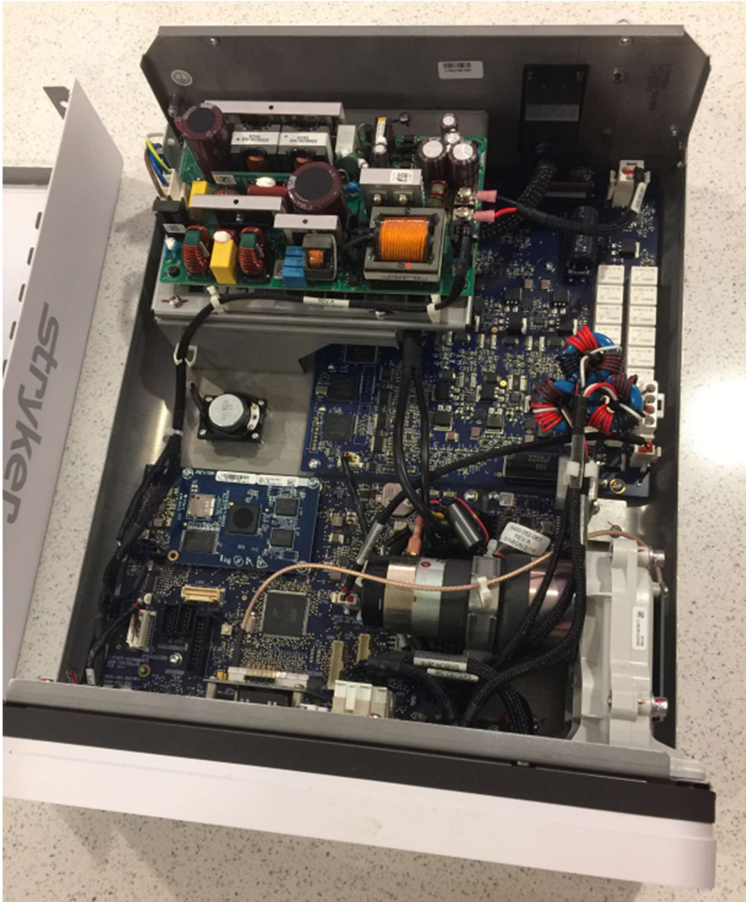
Figure 1. Internal Front View
