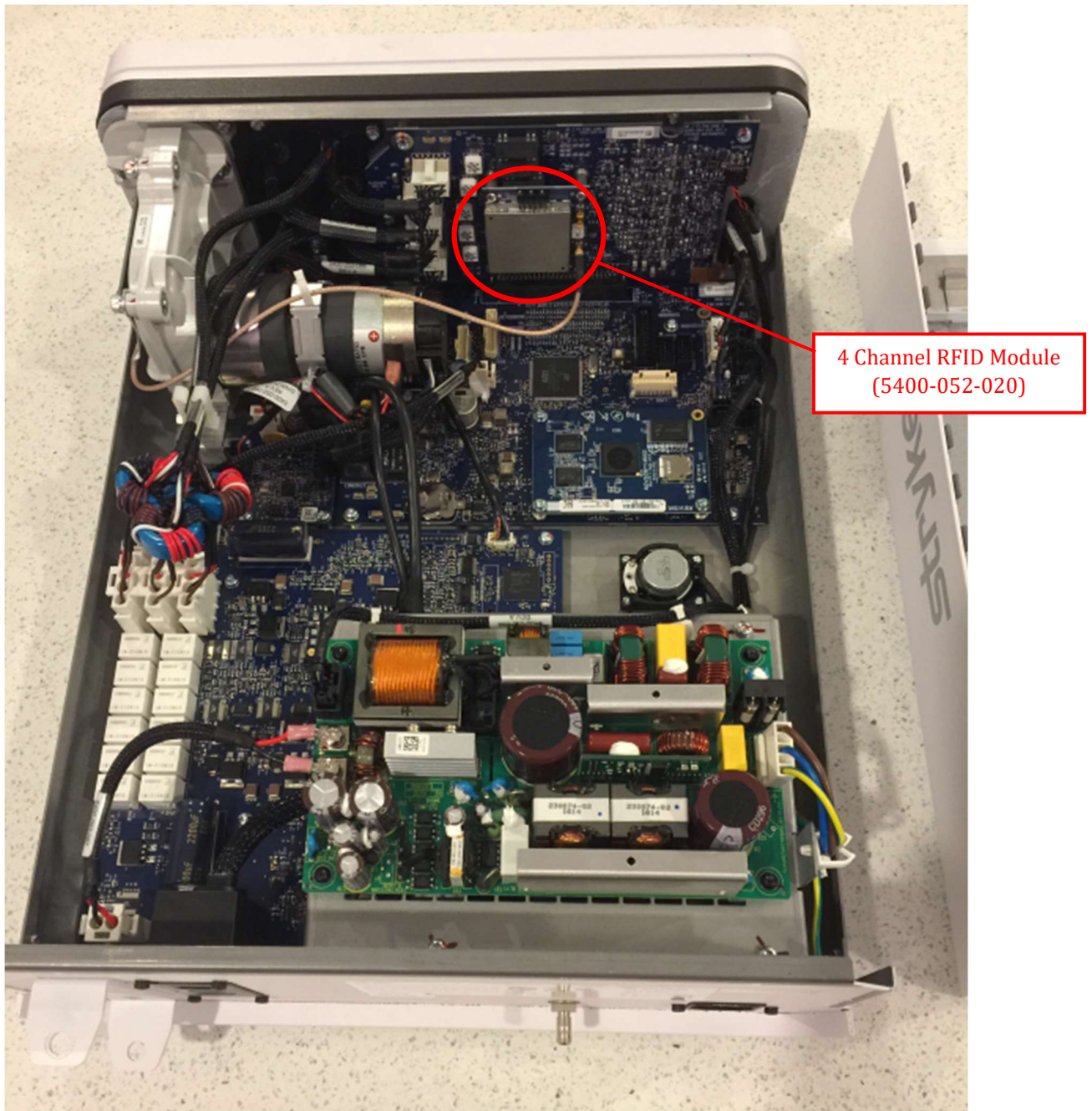
Figure 2. Internal Rear View
