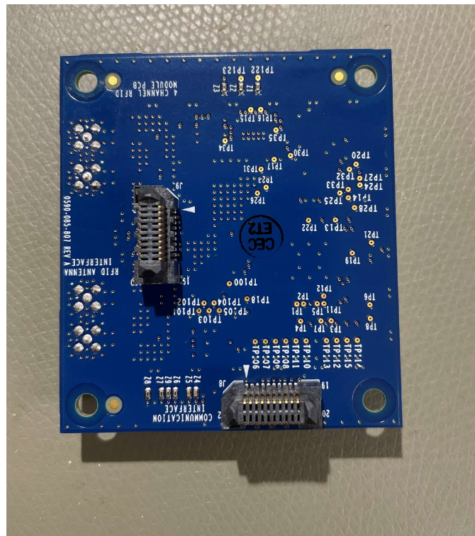
Figure 9. RF Module PCBA Bottom View
