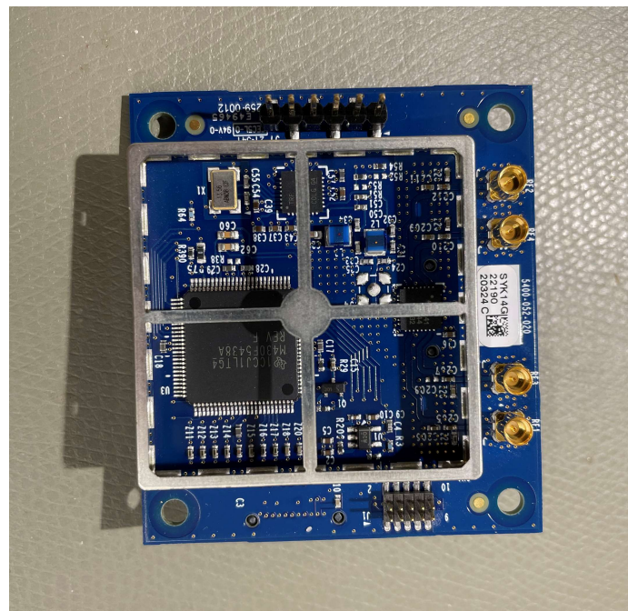
Figure 8. RF Module PCBA Top View without cover
