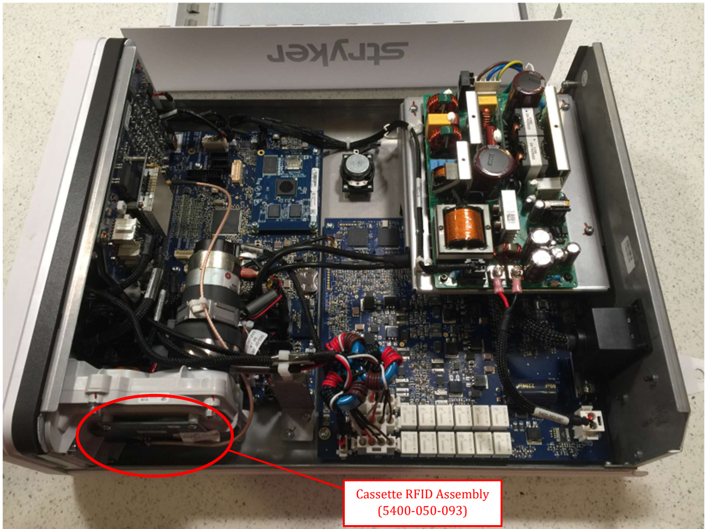
Figure 3. Internal Right View
