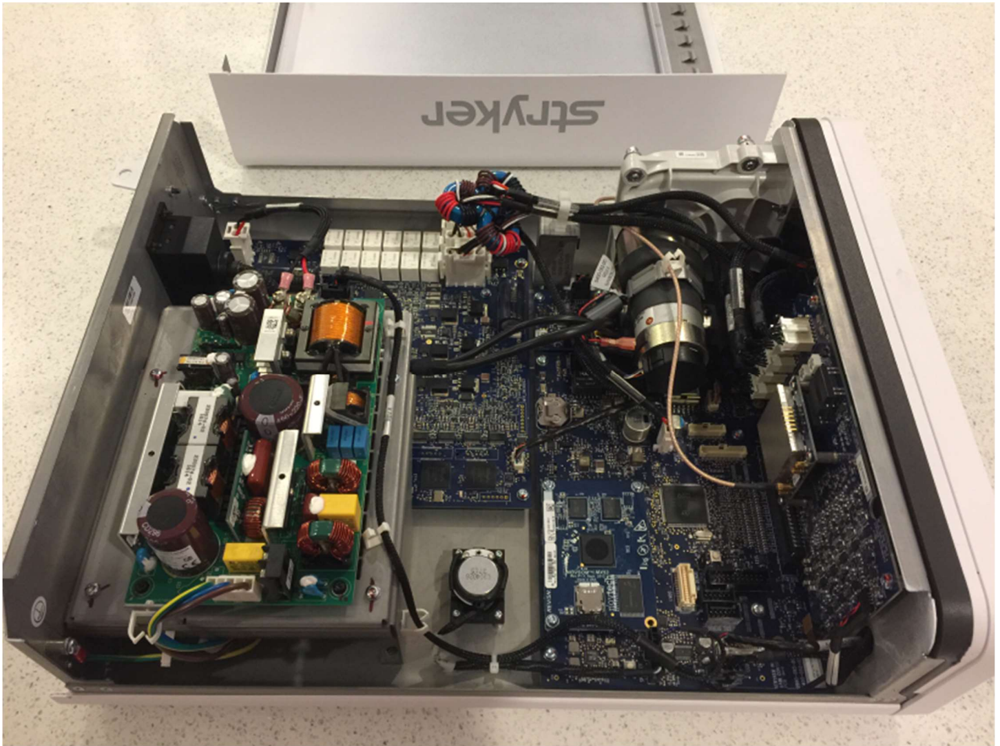
Figure 4. Internal Left View
