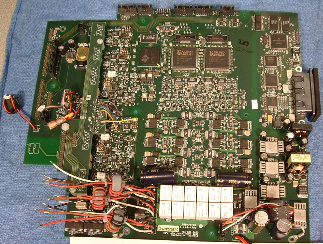
Main PCB
