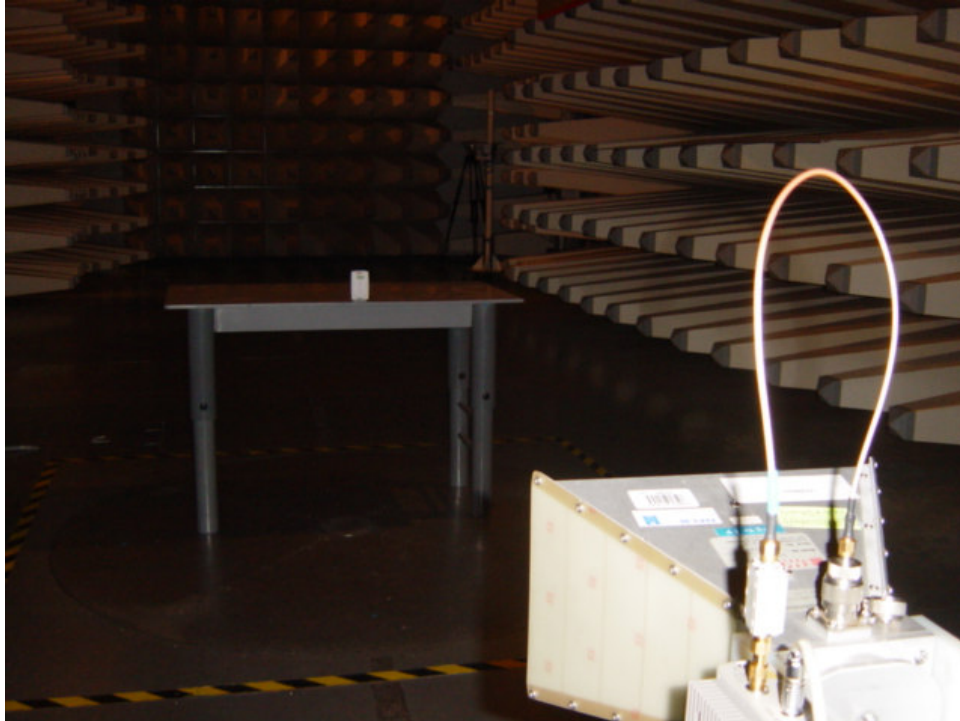
Set up of radiated emission test
