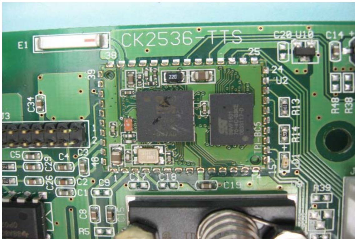
Internal View of EUT(Bluetooth)
