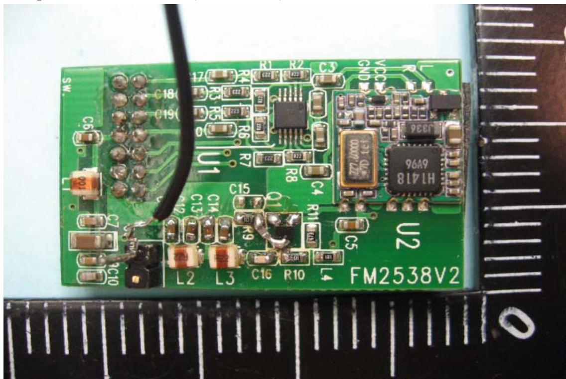
Component View of PCB (FM Module)
