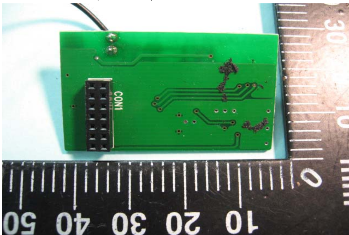
Solder View of PCB (FM Module)
