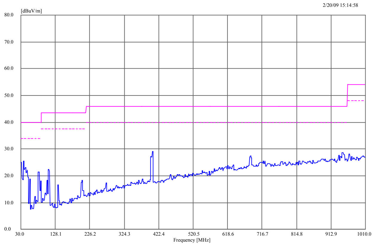
Figure 109: Emissions Pres-can, 10dBi Dipole Antenna, 30 to 1000 MHz, X-Axis
