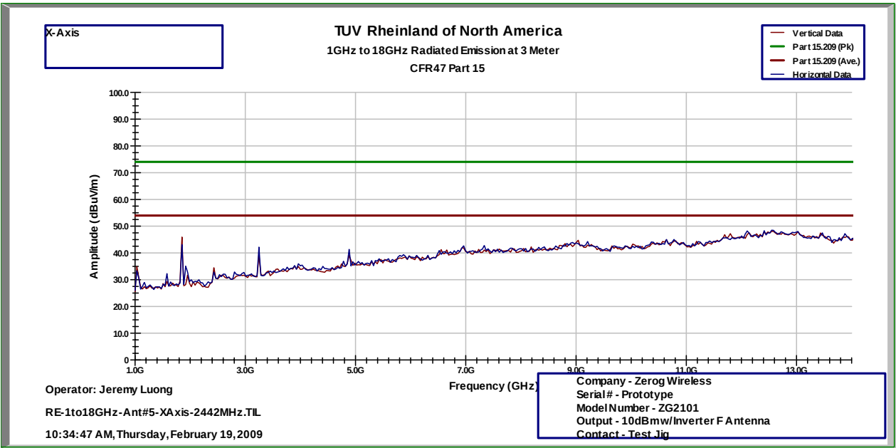
Figure 50: Emissions Pres-can, Inverter F Antenna, 1GHz-18GHz, X-Axis
