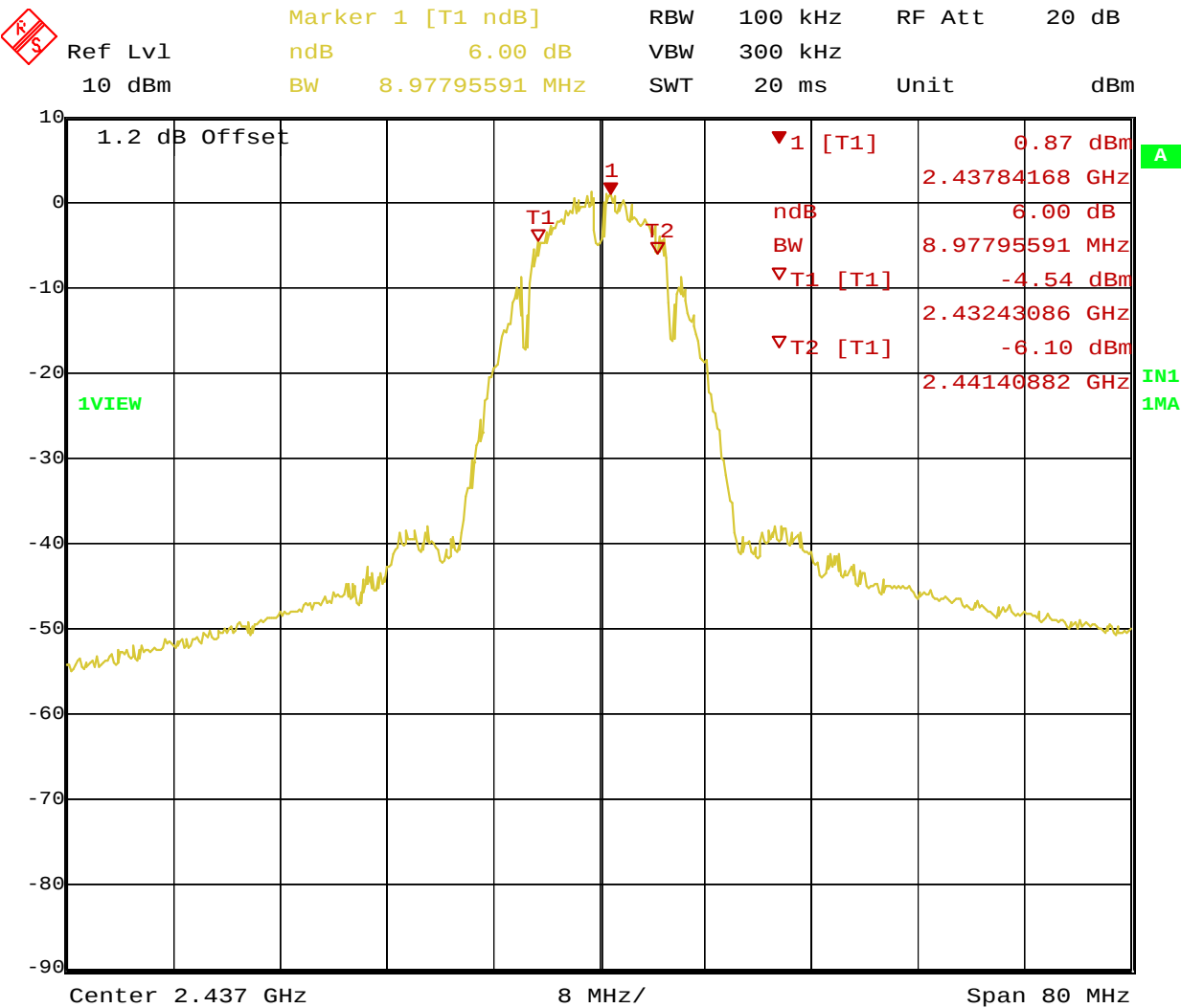
Date: 23.FEB.2009 10:43:40 Figure 11: 6dB Bandwidth – Operating Channel 2437MHz
