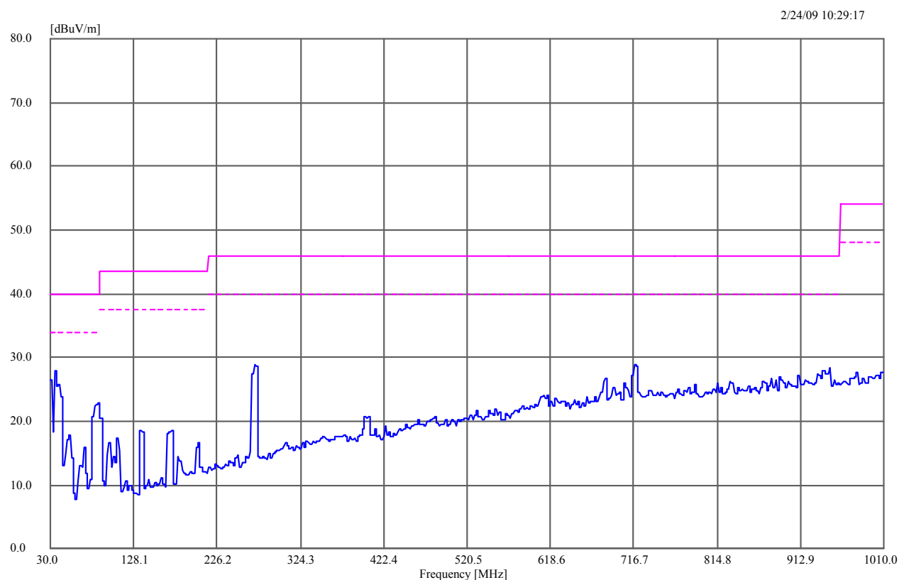
Figure 105: Emissions Pres-can, 5dBi Dipole Antenna, 30 to 1000 MHz, Y-Axis
