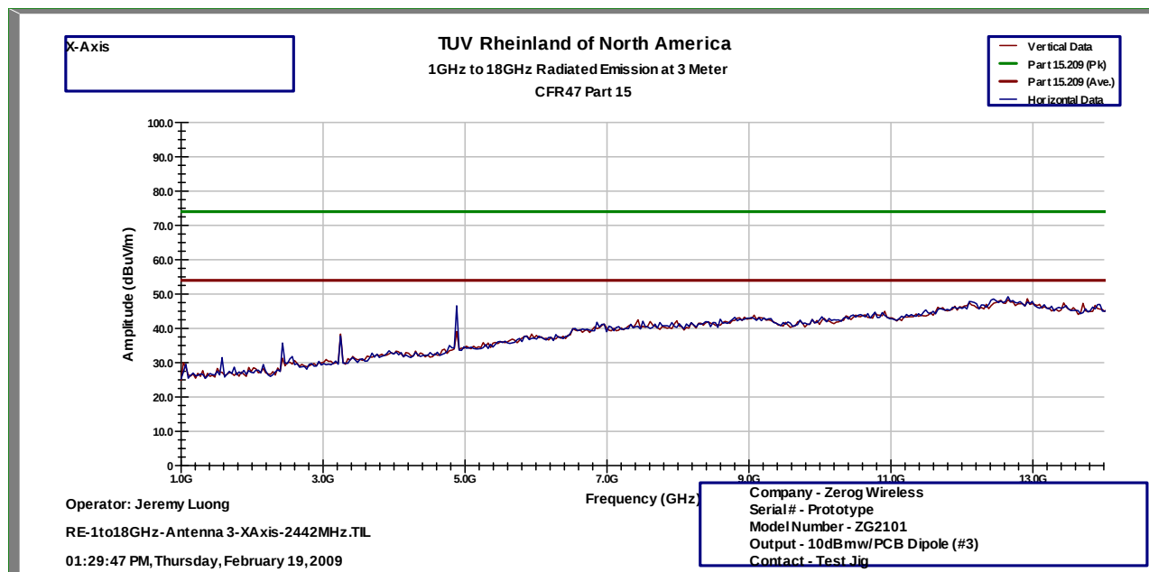
Figure 56: Emissions Pres-can, 2dBi PCB Antenna #3, 1GHz-18GHz, X-Axis
