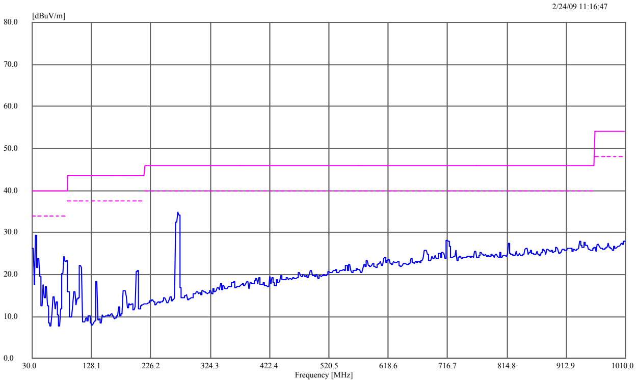
Figure 41: Emissions Pres-can, 2dBi Dipole Antenna (RFA-02-D3-70-100), 30 to 1000 MHz, Z-Axis
