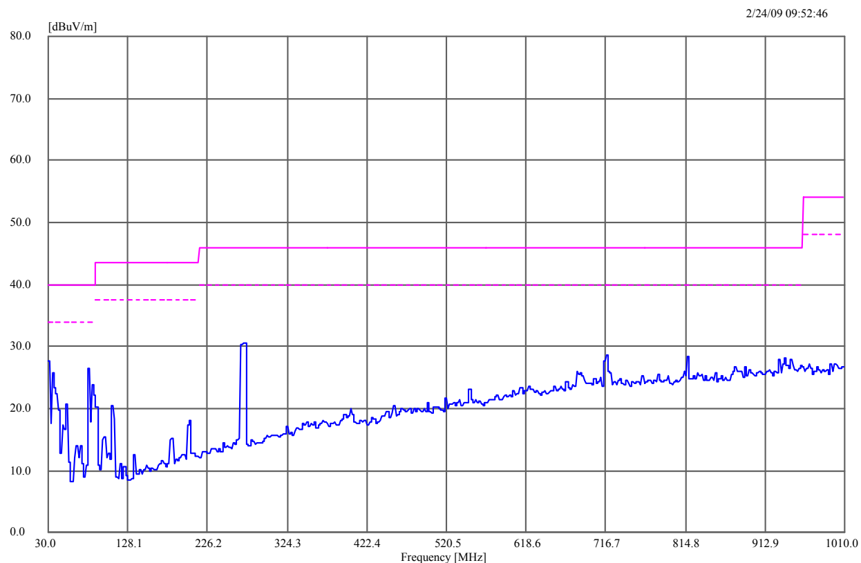
Figure 99: Emissions Pres-can, 2dBi PCB Antenna #3, 30 to 1000 MHz, Y-Axis
