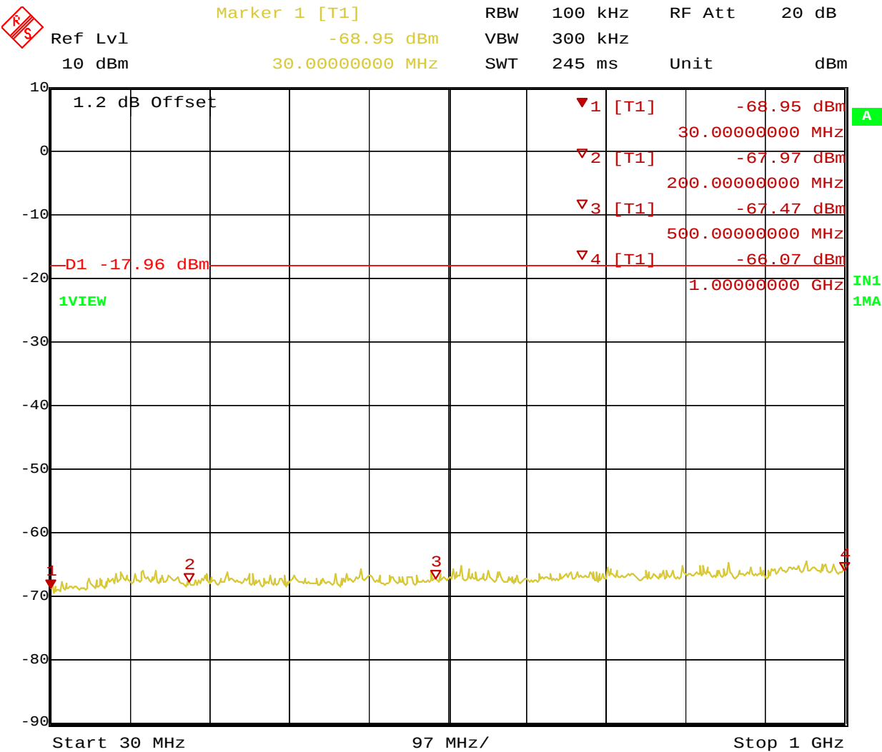
Figure 24: Band-edge Requirement for Operating Channel 2462MHz (30MHz to 1GHz)
