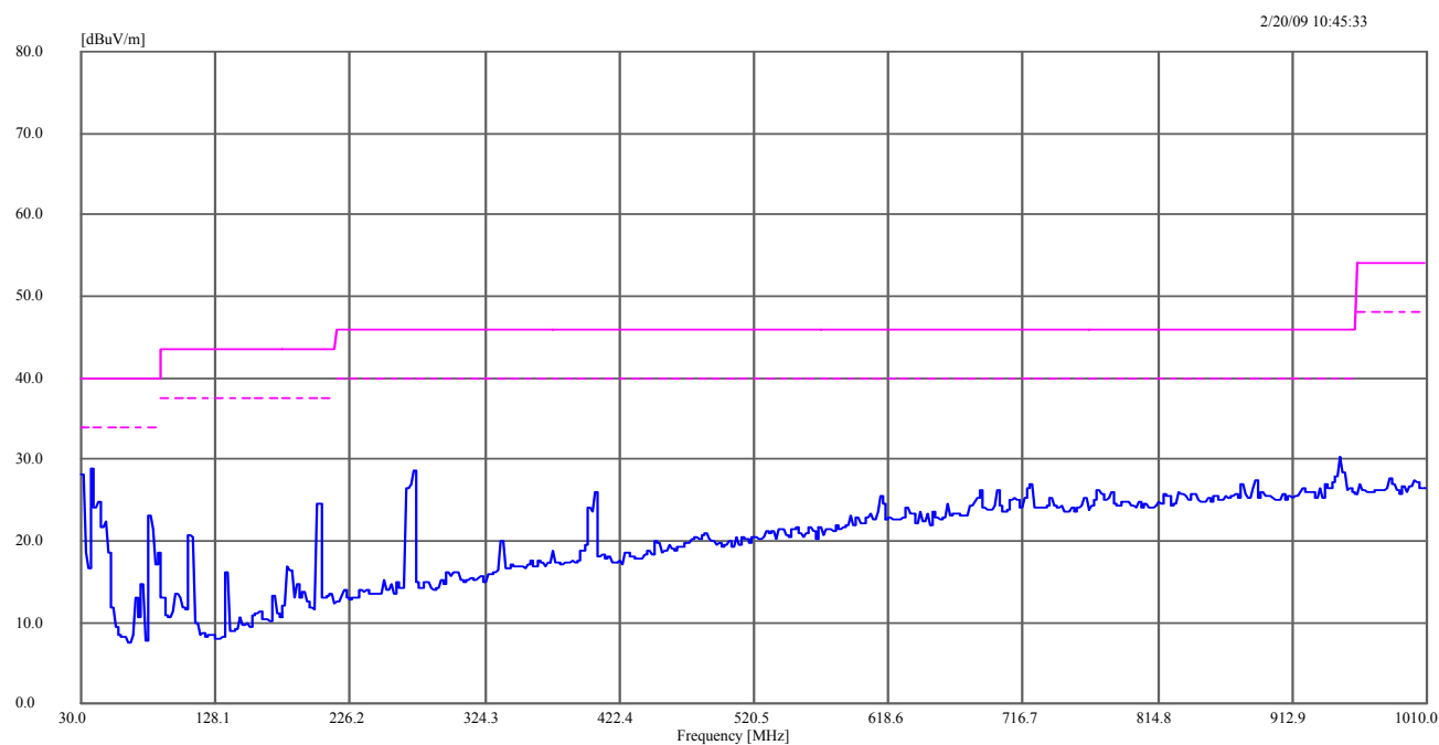
Figure 43: Emissions Pres-can, Helical Antenna, 30 to 1000 MHz, X-Axis
