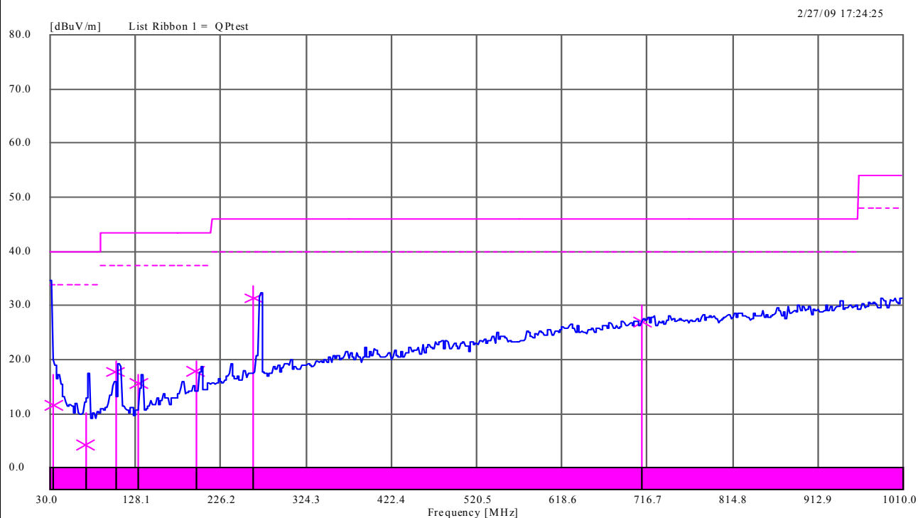
30MHz to 1000MHz Plot for Transmit Mode at 2462MHz
