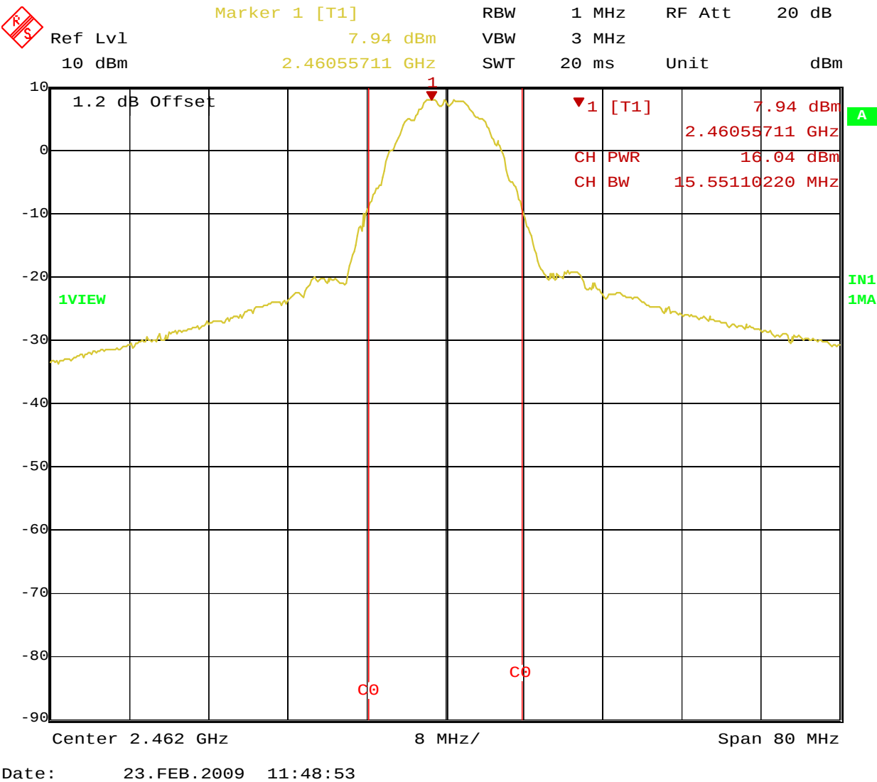
Figure 3: Maximum Transmitted Power at 3.3VDC – Highest Channel 2462 MHz
