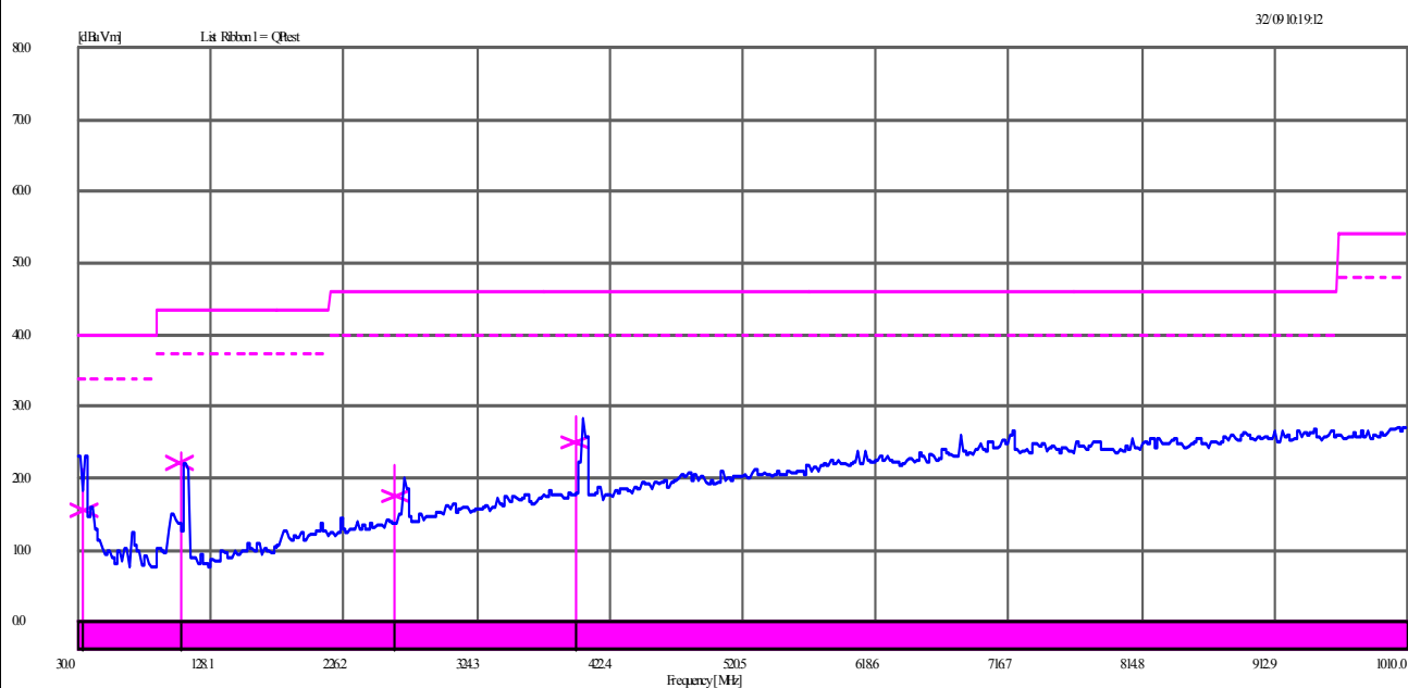
30MHz to 1000MHz Plot for Transmit Mode at 2437MHz
