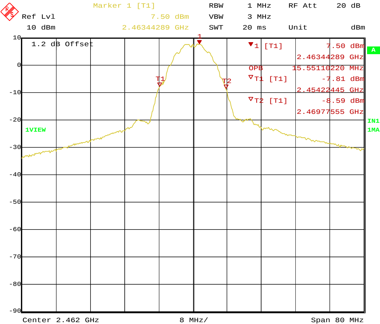
Date: 23.FEB.2009 11:37:48 Figure 15: 99% Bandwidth – Operating Channel 2462MHz
