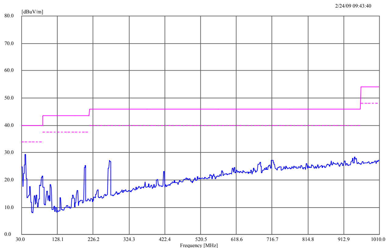
Figure 97: Emissions Pres-can, 2dBi PCB Antenna #3, 30 to 1000 MHz, X-Axis
