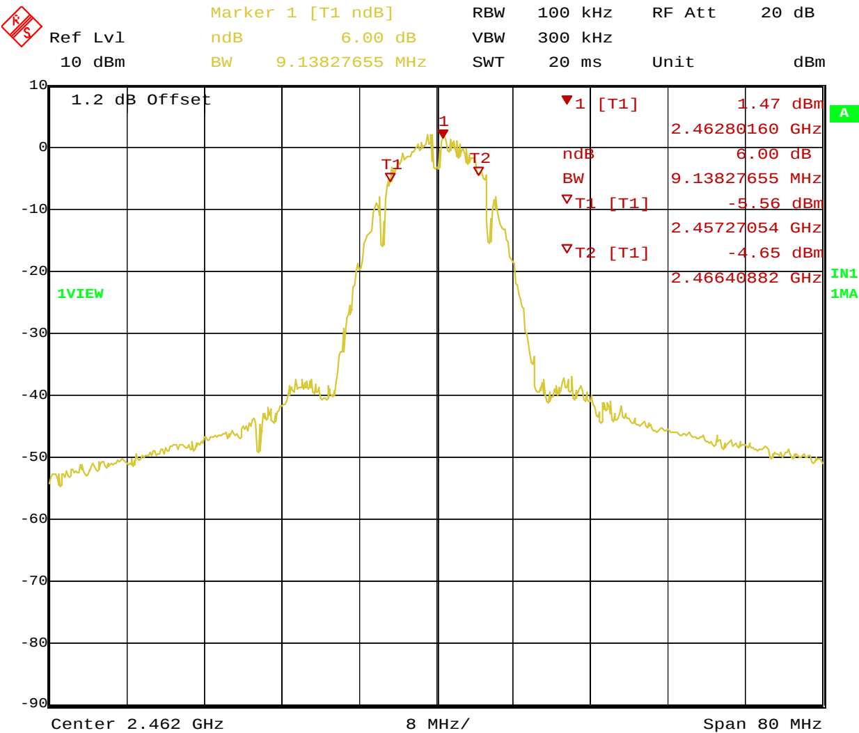
Date: 23.FEB.2009 11:40:44 Figure 12: 6dB Bandwidth – Operating Channel 2462MHz
