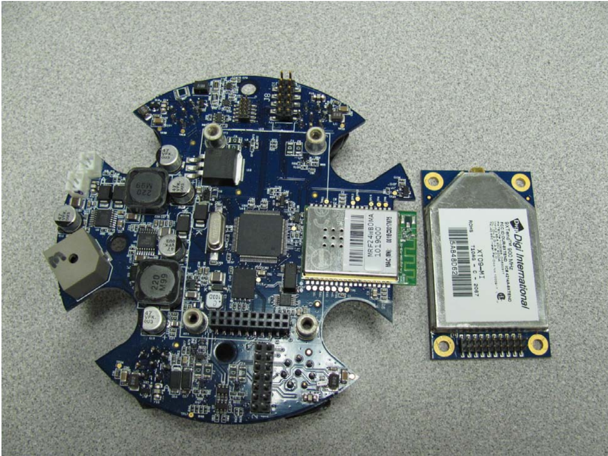
Node PCB Disassembled
