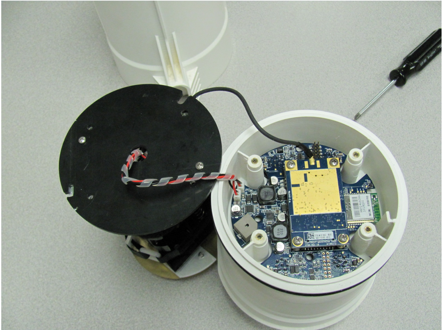
TruBlue(TM) Remote Monitoring System Node internal view
