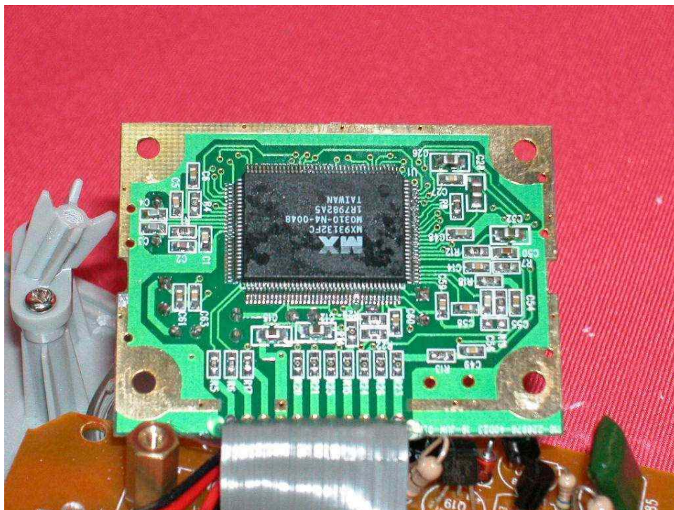
Base DAM main IC PCB front side
