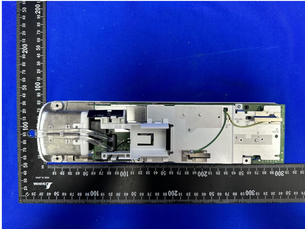
(4) EUT Photo – ASIN0305
