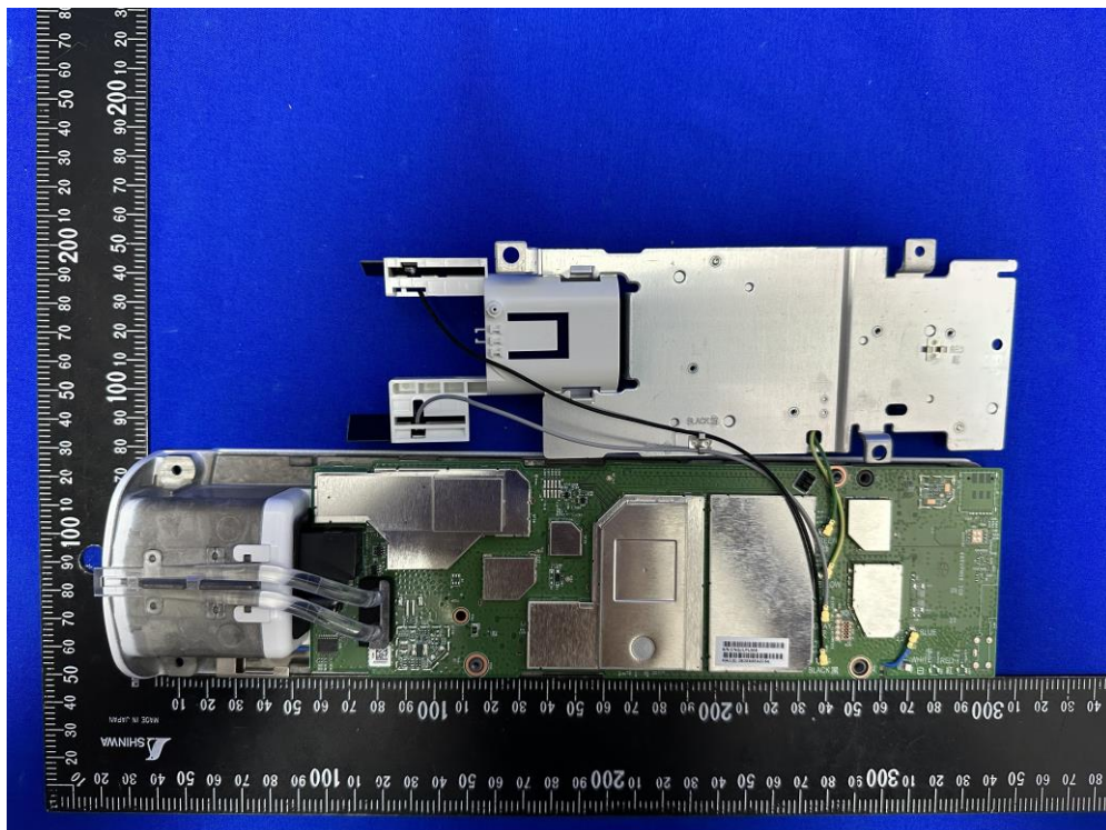
(5) EUT Photo – ASIN0305
