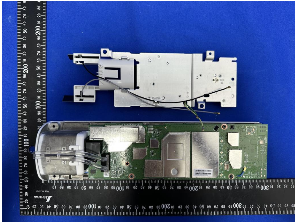
(6) EUT Photo – ASIN0305
