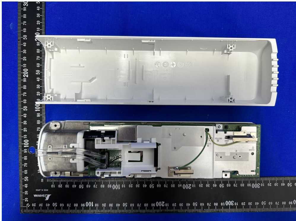
(2) EUT Photo – ASIN0305
