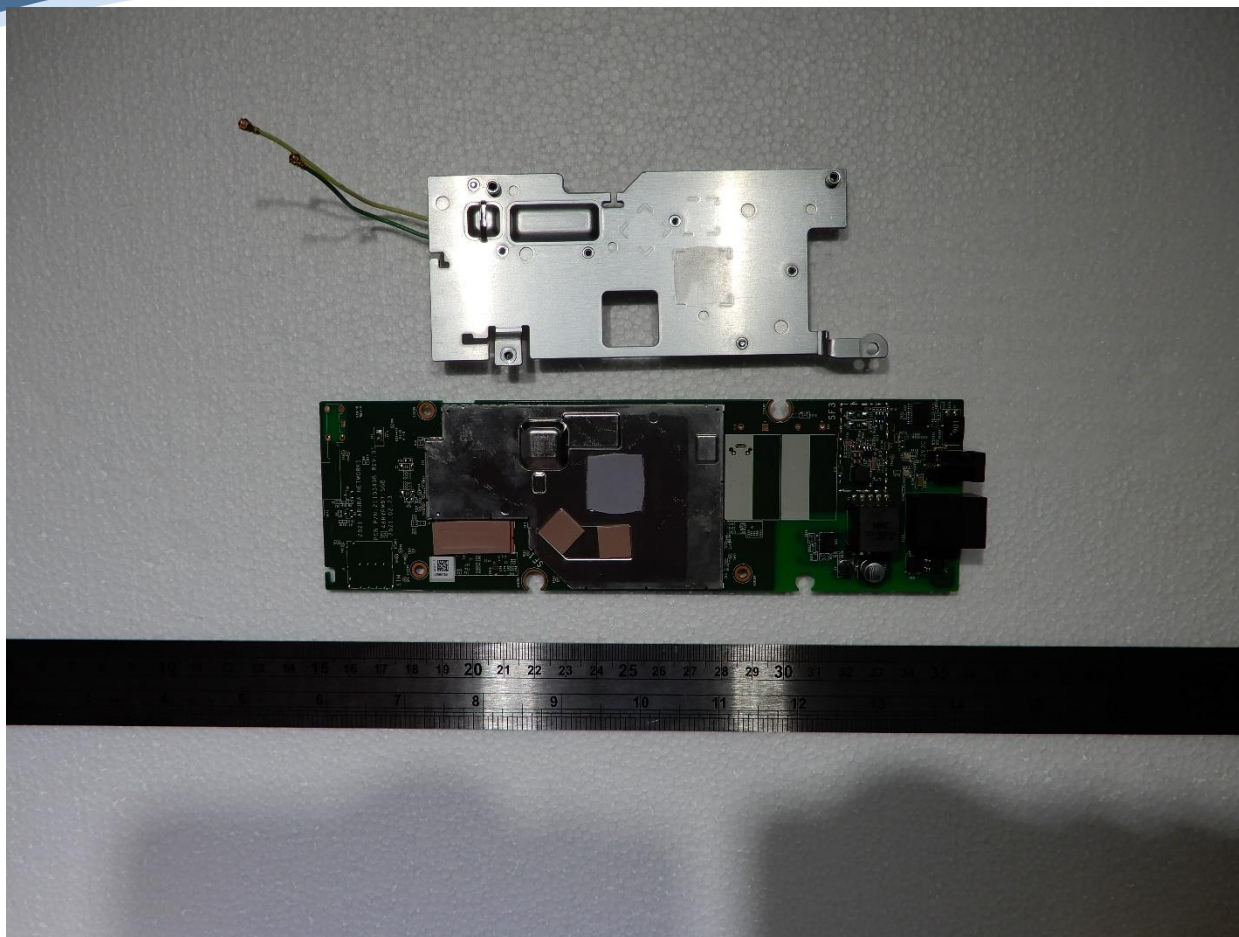
Main Board Top Heatsink Removed
