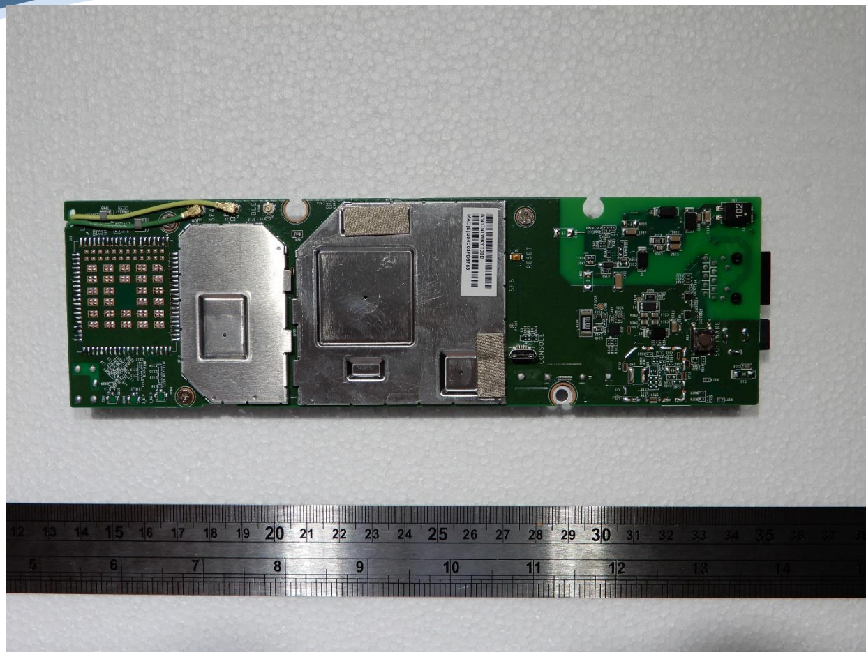
Main Board Bottom
