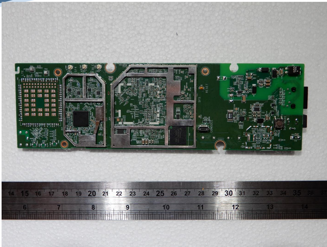
Main Board Bottom Shields Removed
