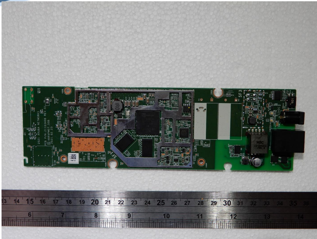
Main Board Top Shields Removed
