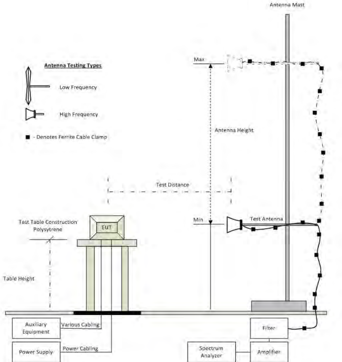
Radiated Emission Test Setup
