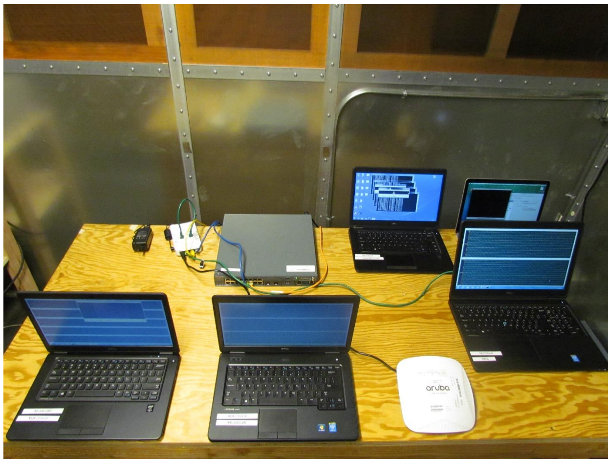
Conducted Emissions ACDC configuration Front View
