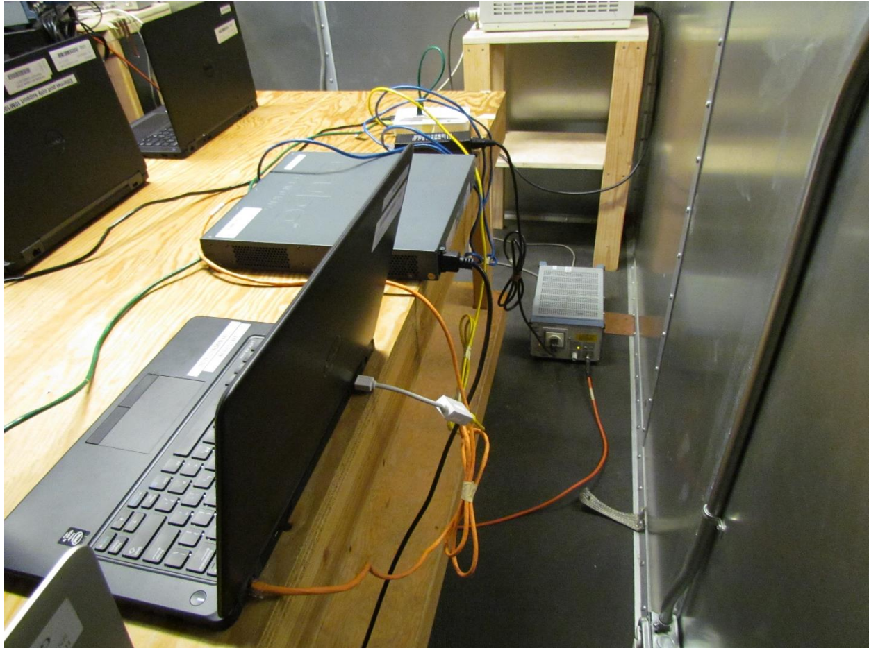
Conducted Emissions PoE configuration Rear View
