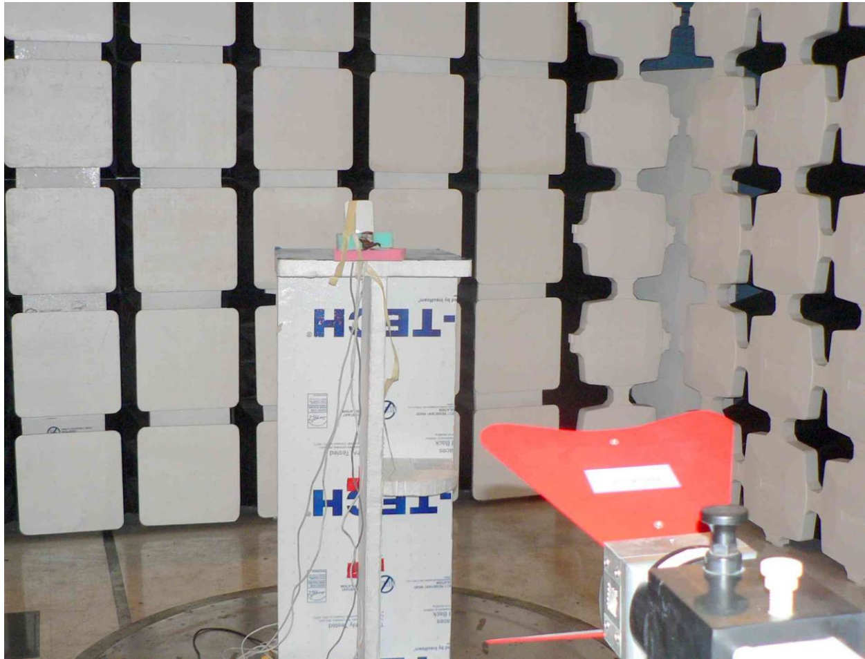
HWPDP85 Wi-Fi TX Spurious
