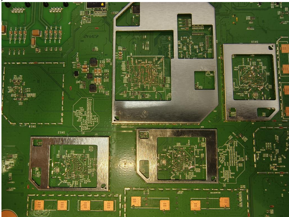
(38) EUT Photo
