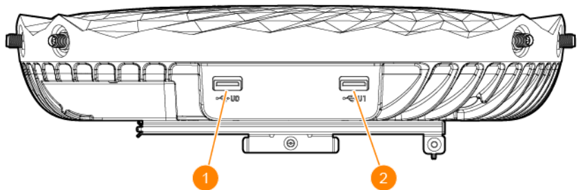
Figure 4 AP-754 Access Point Side A View
