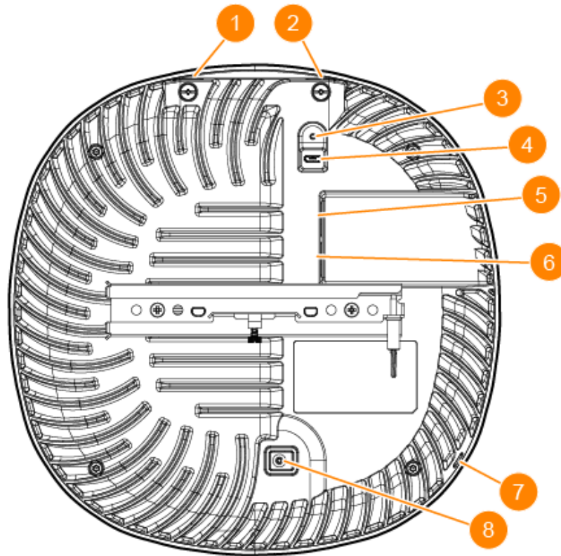
Figure 3 AP-735/AP-735A Back View
