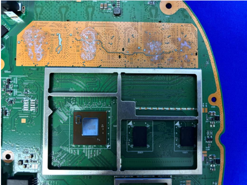
(11) EUT Photo (Model: APIN0735A)
