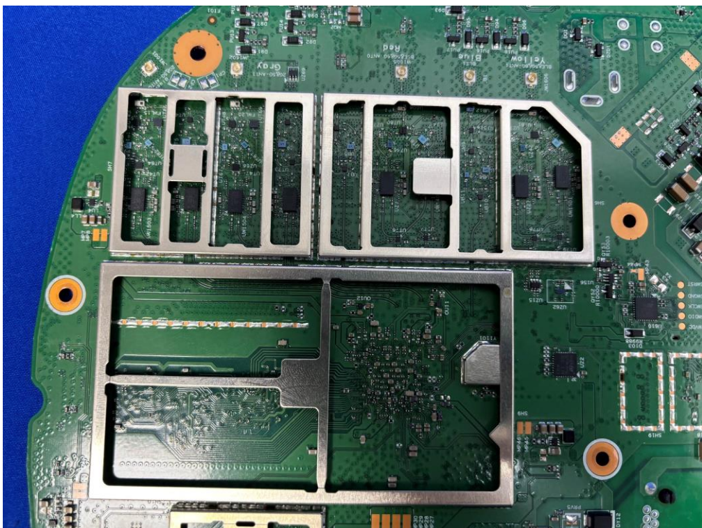
(10) EUT Photo (Model: APIN0735A)
