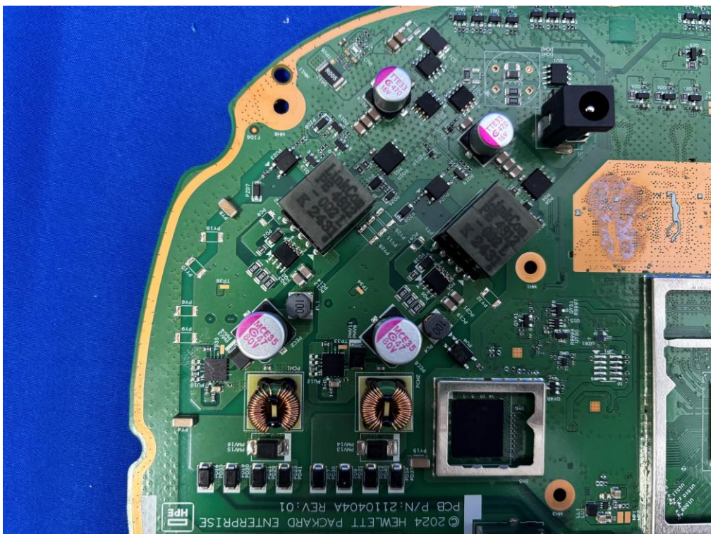
(8) EUT Photo (Model: APIN0735A)
