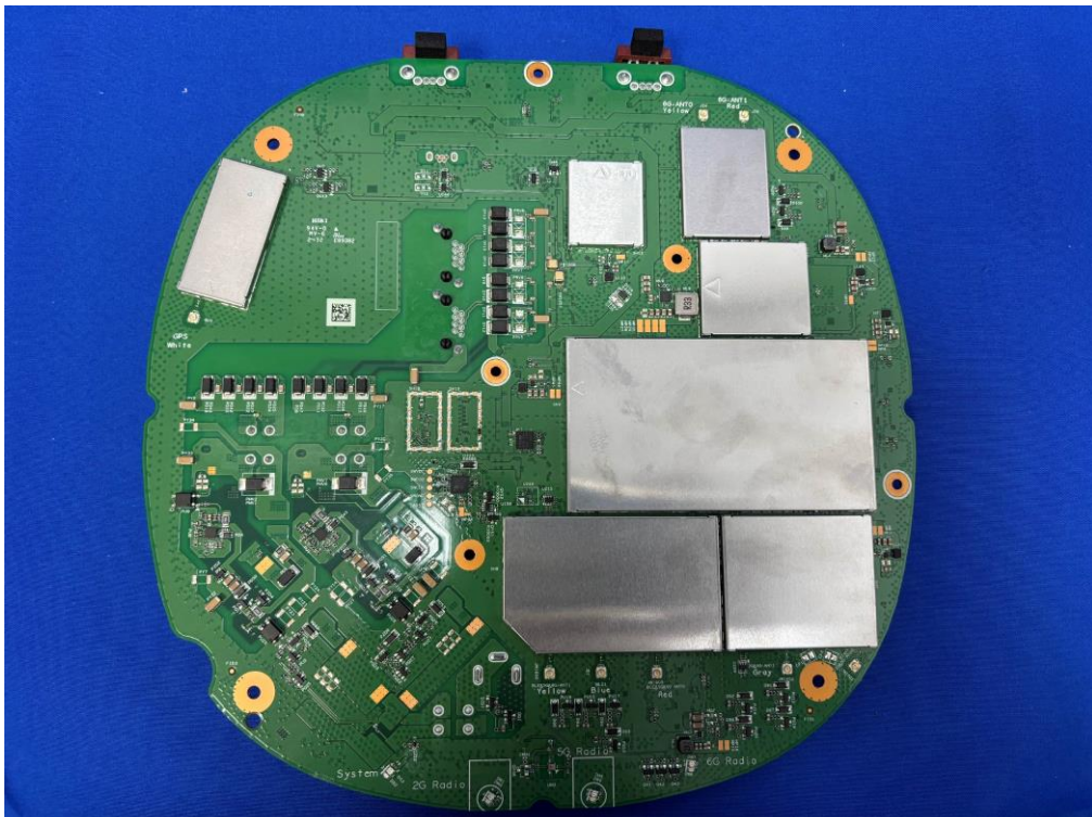
(4) EUT Photo (Model: APIN0735A)
