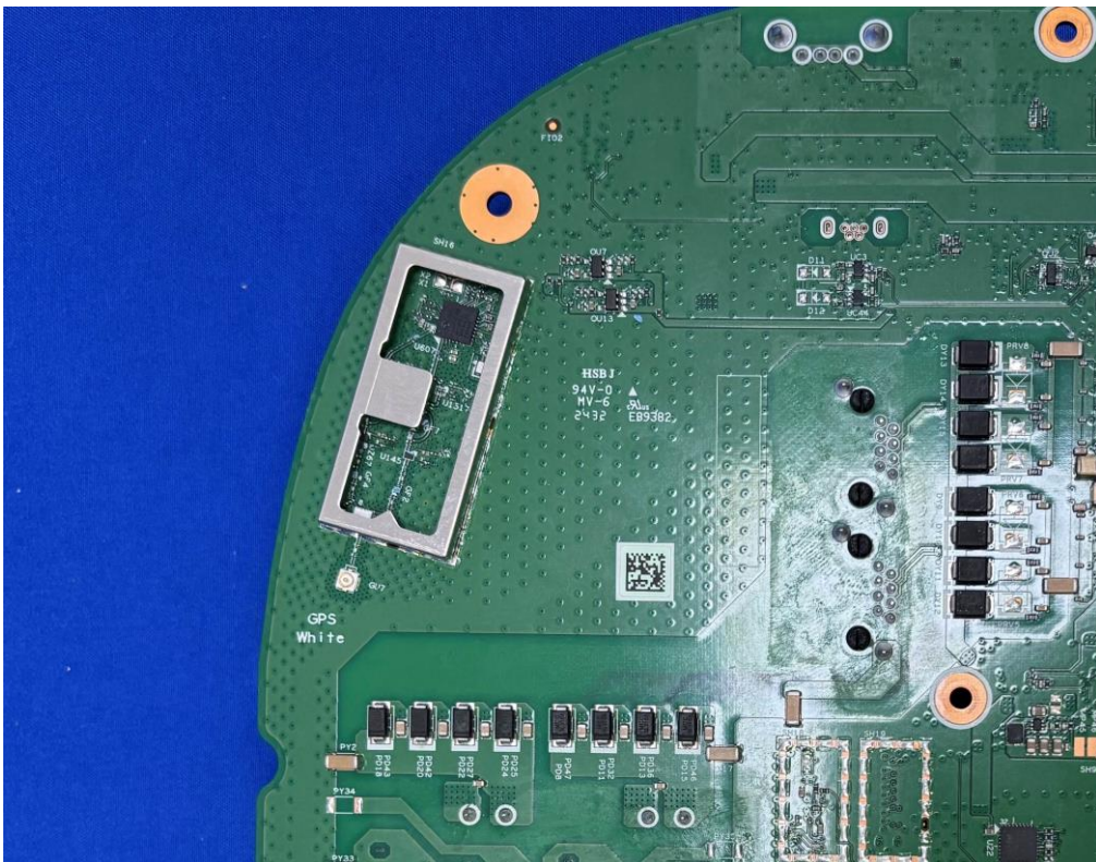
(12) EUT Photo (Model: APIN0735A)
