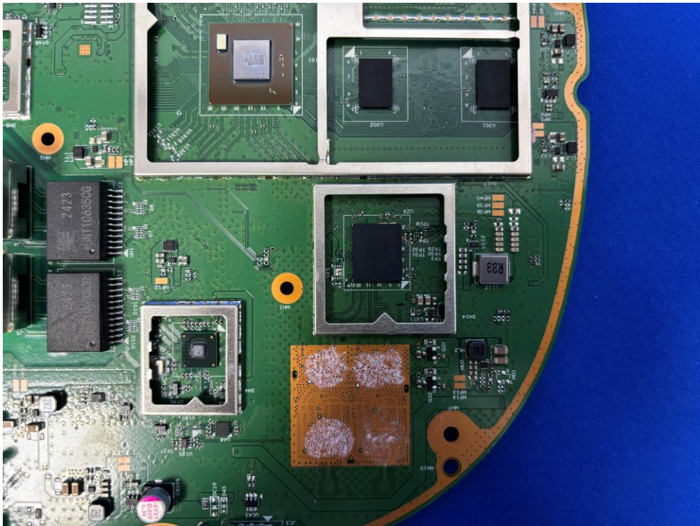
(7) EUT Photo (Model: APIN0735A)
