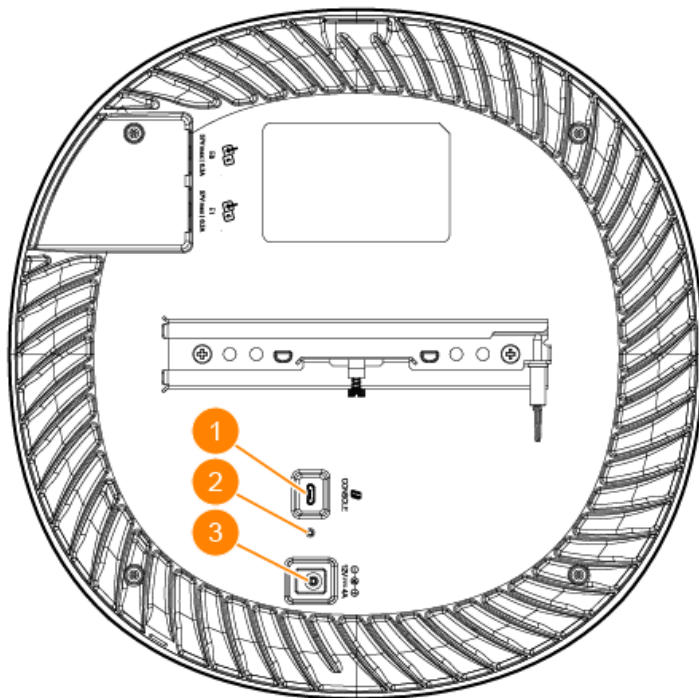
Figure 7 AP-655 Access Point Rear View
