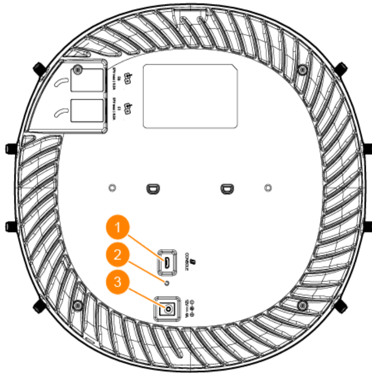
Figure 8 AP-654 Access Point Rear View
