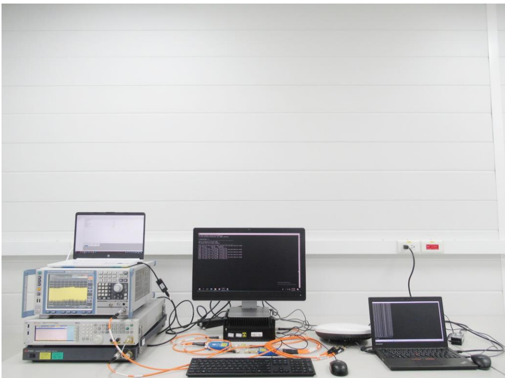
Description: DFS Test Setup _ Conducted
