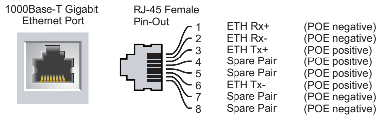
Figure 5 Ethernet Port Pin-Out
