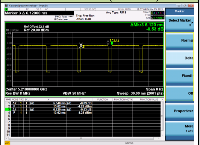
802.11ac-VHT80 (T=5.340ms)
