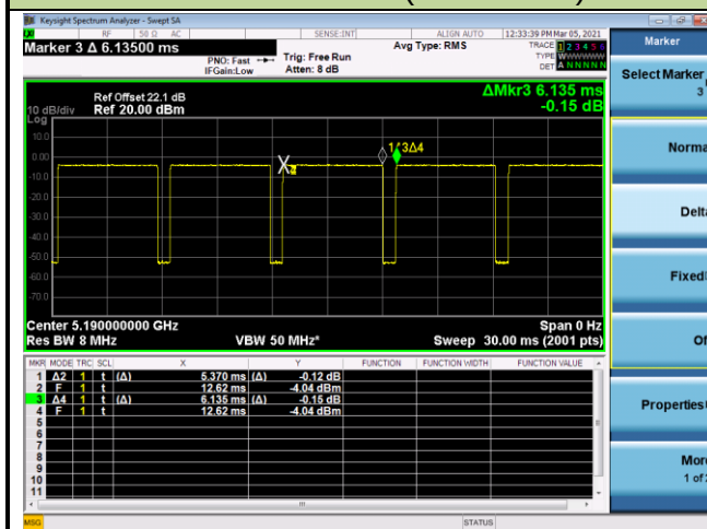
802.11ac-VHT40 (T=5.370ms)
