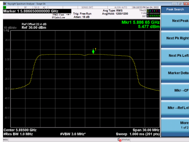
Channel 177 (5885MHz)
