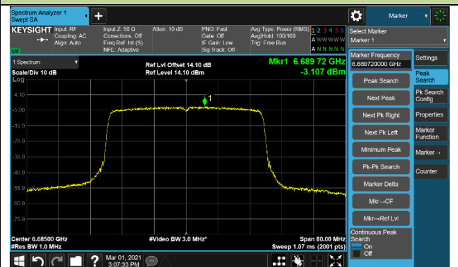
Channel 147 (6685MHz)
