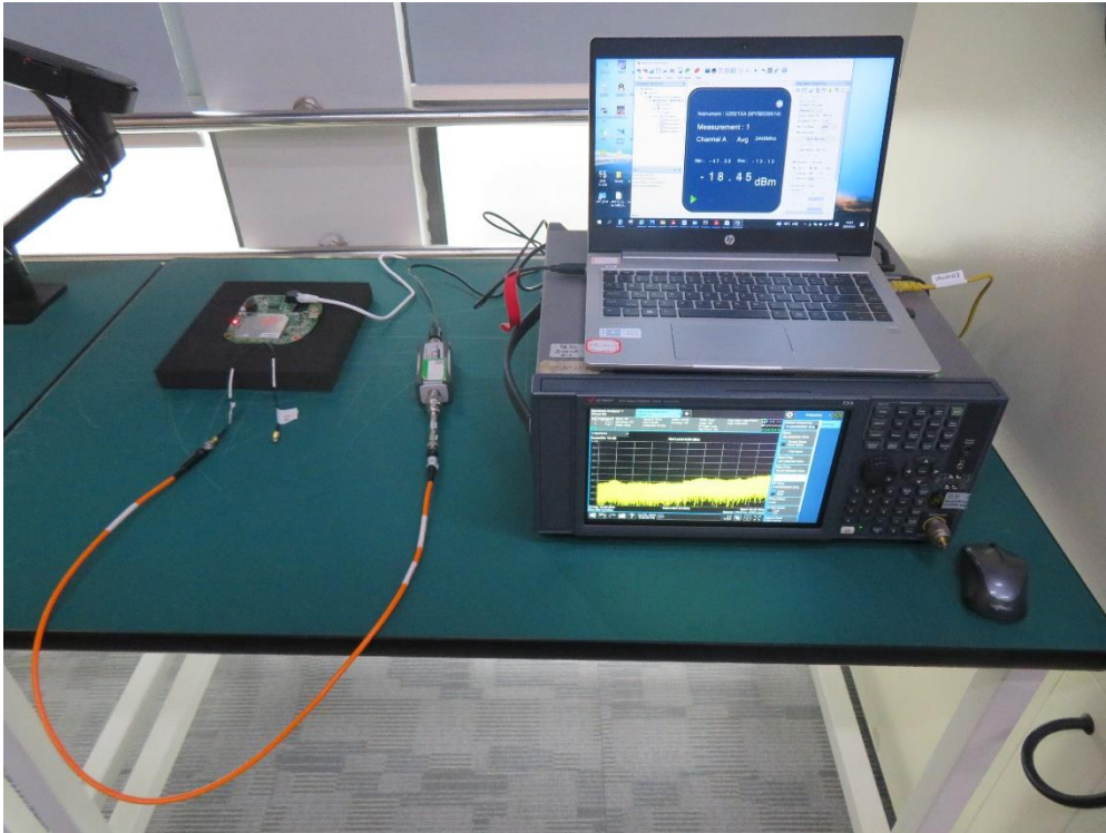
Description: DFS Conducted Measurement Test Setup
