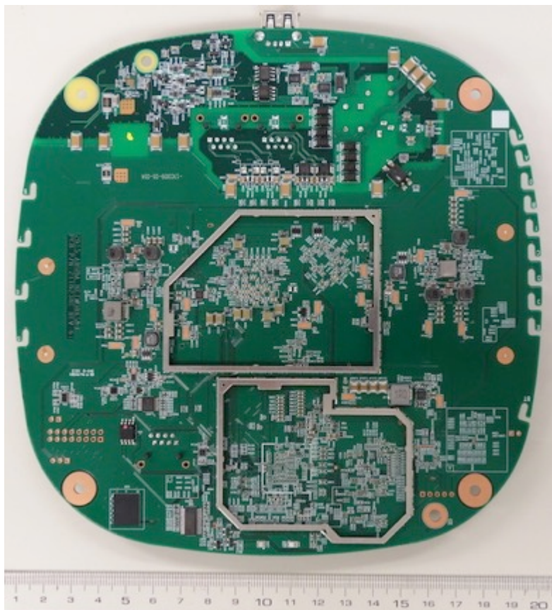
PCB - Bottom with Shield Removed
