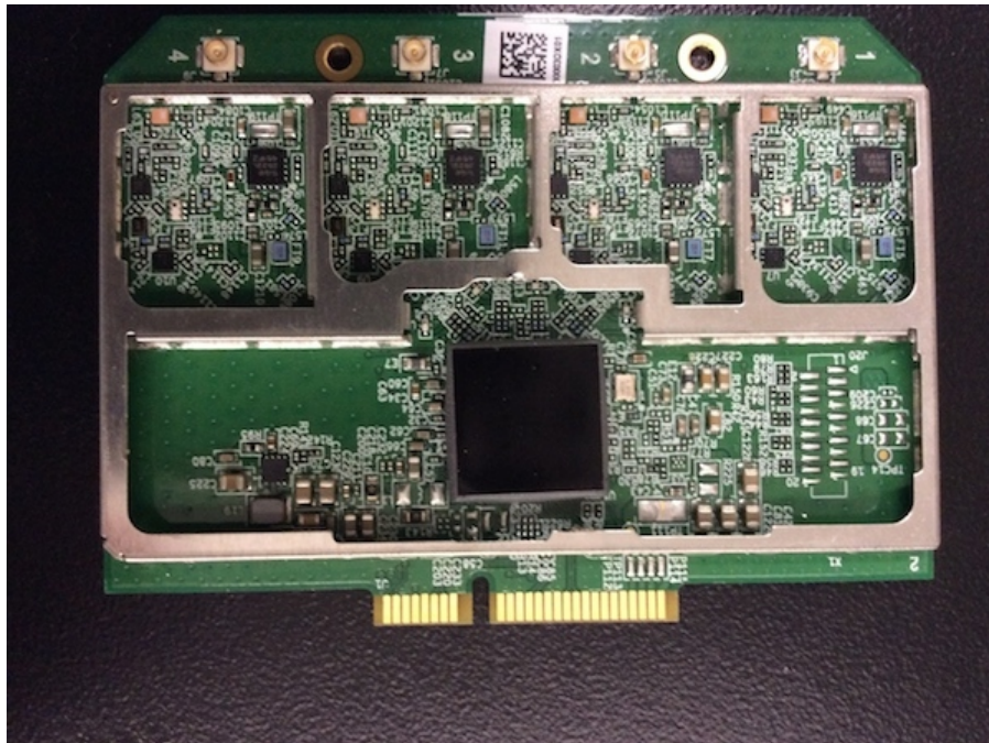
2.4GHz Card (Top – Shield Removed)
