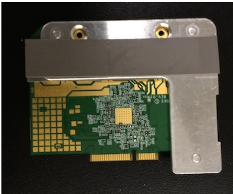
2.4Ghz Card (Bottom View)
