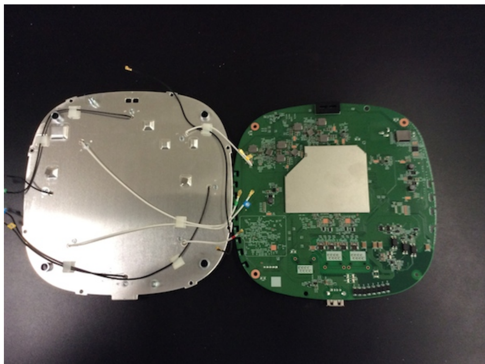
View under Antenna Plate
