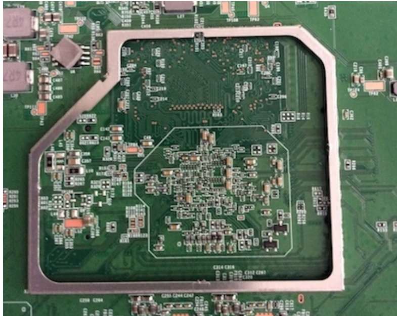
Close-Up Main Board CPU Shield Removed
