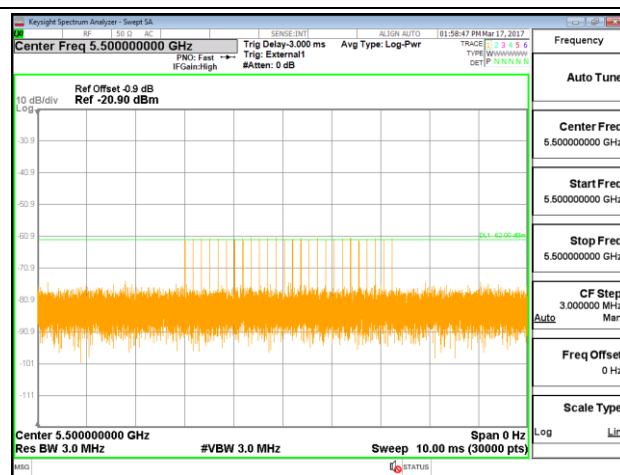
Radar Type 4
