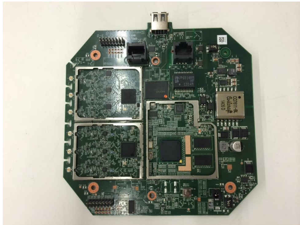
TOP OF PCB WITHOUT SHIELDS
