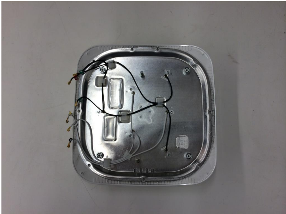
INSIDE OF TOP COVER SHOWING INTERNAL ANTENNAS
