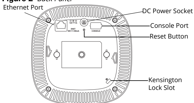
Figure 2 Back Panel
