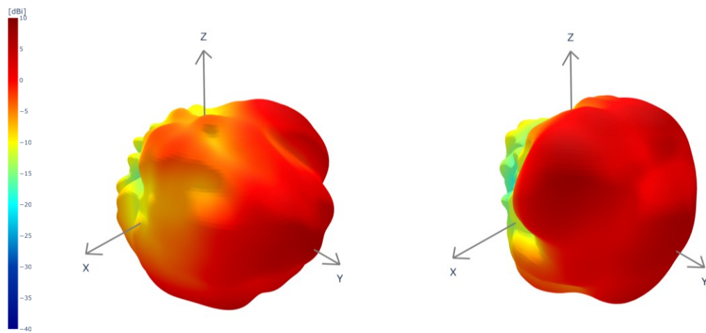
5.2GHz Wi-Fi antenna patterns
