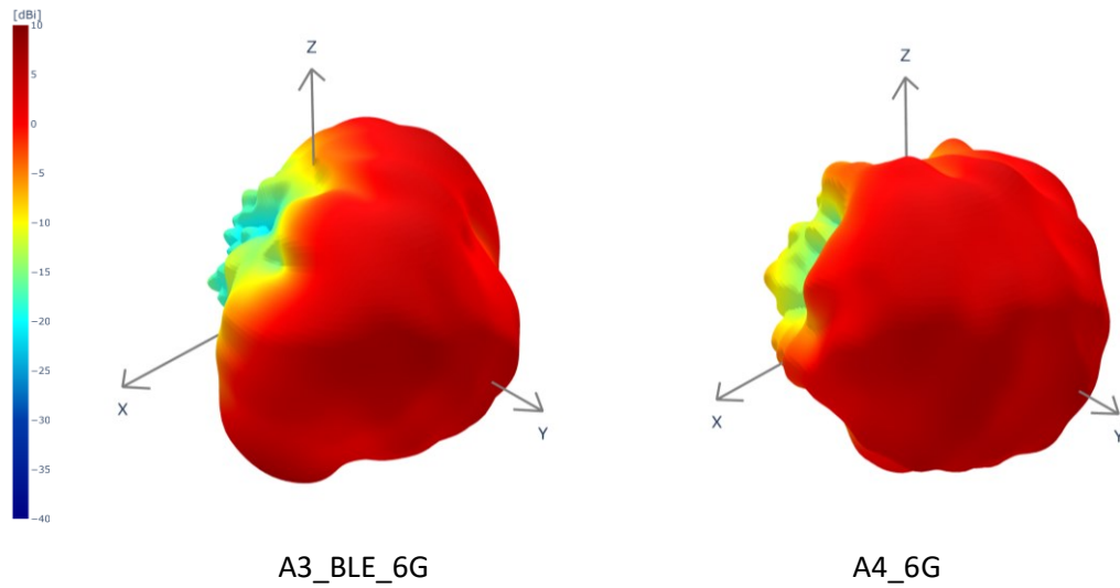
6.9GHz Wi-Fi antenna patterns
