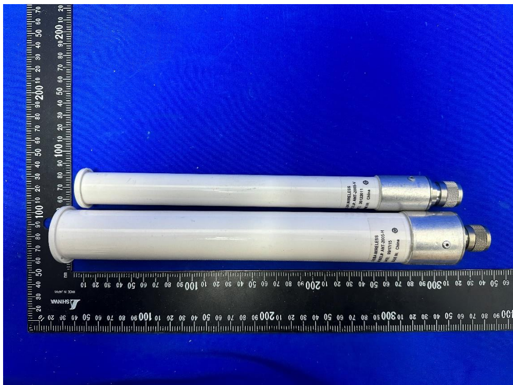
(10) EUT Photo - (ANT-2x2-5005-H and ANT-2x2-5005-V)
