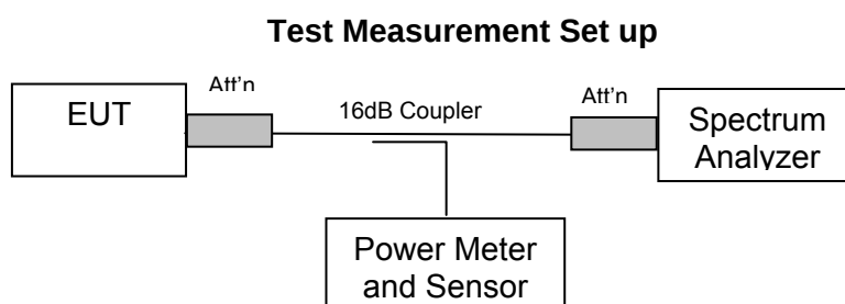
Test set up for Occupied Bandwidth and Emission Mask measurement
