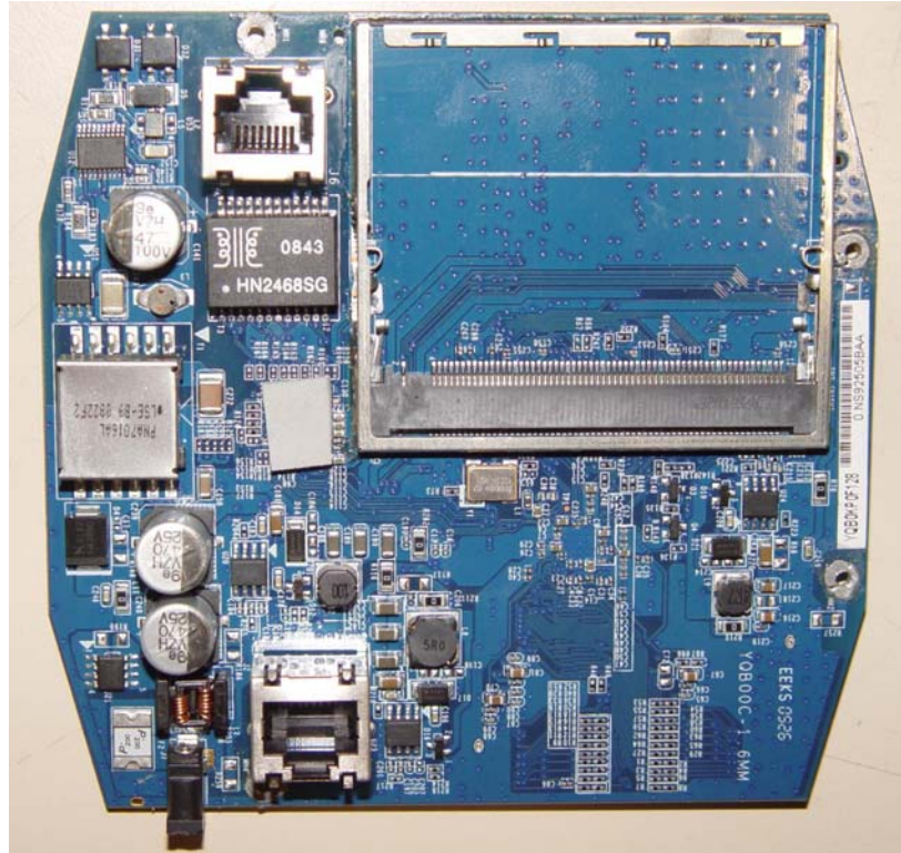
Main Assembly Top
