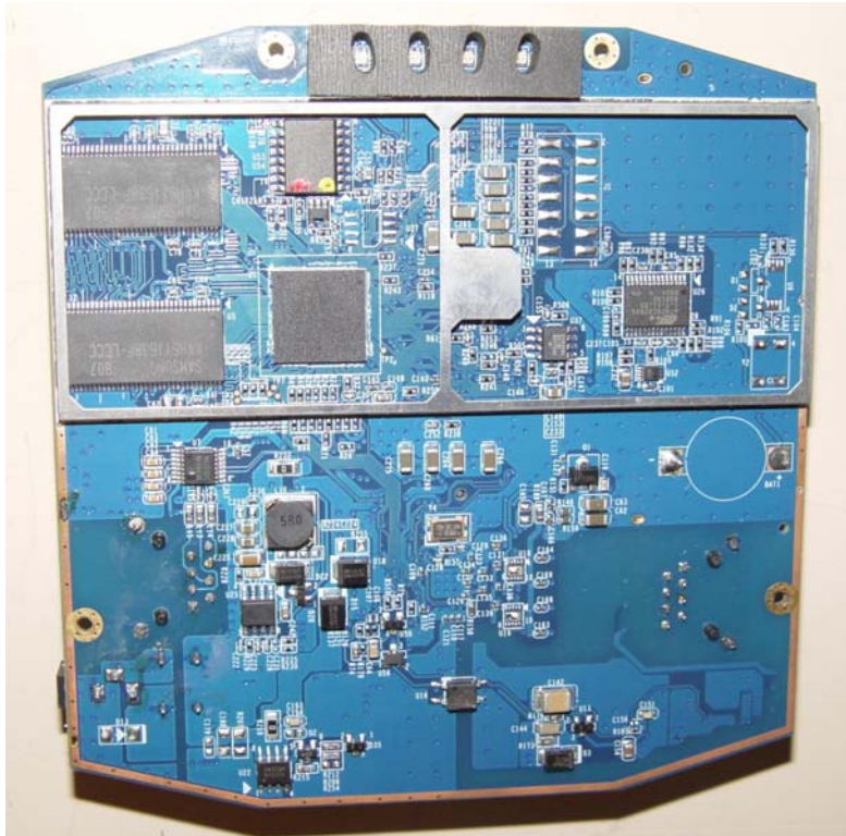
Main Assembly Bottom
