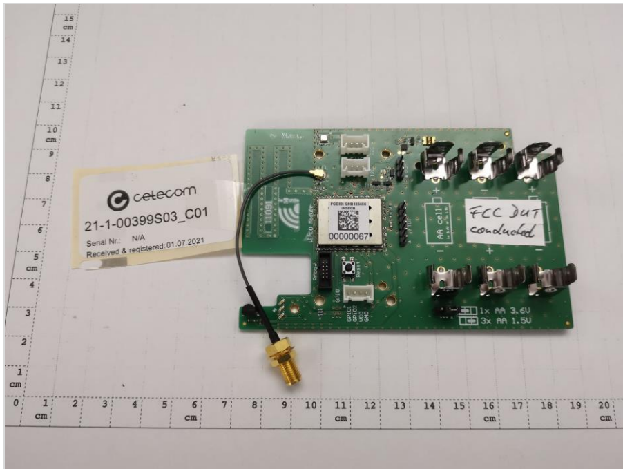
Photograph 3: EUT 2_Top view
